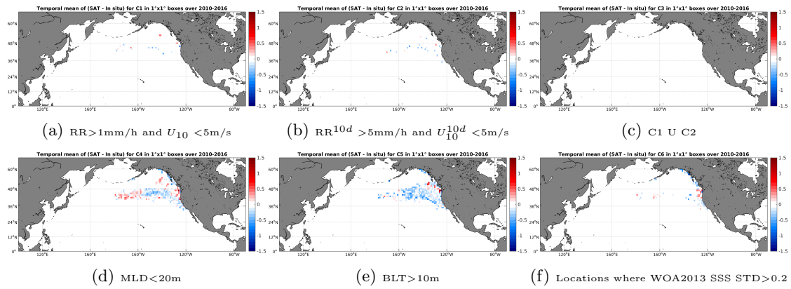
Figure 12: Temporal mean gridded over spatial boxes of size 1^\circ \times 1^\circ of \Delta SSS (SMOS-L3-BEC-OA-V1-9DAYS-0.25DEG - Sea mammals) for 6 different subdatasets corresponding to:RR>1mm/h and U_{10} < 5m/s (a), RR^{10d} > 5mm/h and U_{10}^{10d} < 5m/s (b), C1 U C2 (c),MLD<20m (d),BLT>10m (e),Locations where WOA2013 SSS STD>0.2 (f).
