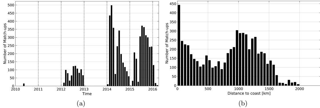
Figure 1: Number of match-ups between Sea mammals and SMOS-L3-BEC-OA-V1-9DAYS-0.25DEG SSS as a function of time (a) and as function of the distance to coast (b) over the North Pacific Ocean Pi-MEP region and for the full satellite product period.
