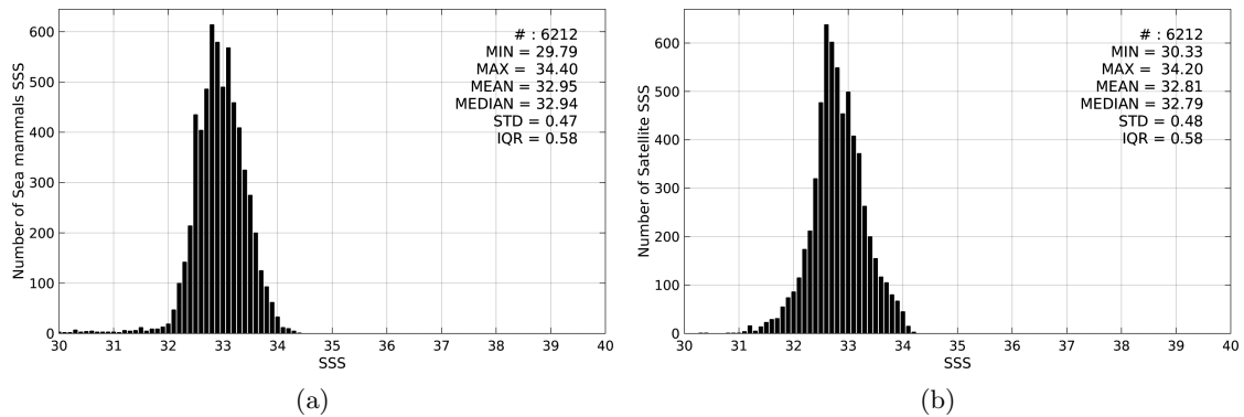
Figure 2: Histograms of SSS from Sea mammals (a) and SMOS-L3-BEC-OA-V1-9DAYS-0.25DEG (b) considering all match-up pairs per bins of 0.1 over the North Pacific Ocean Pi-MEP region and for the full satellite product period.
