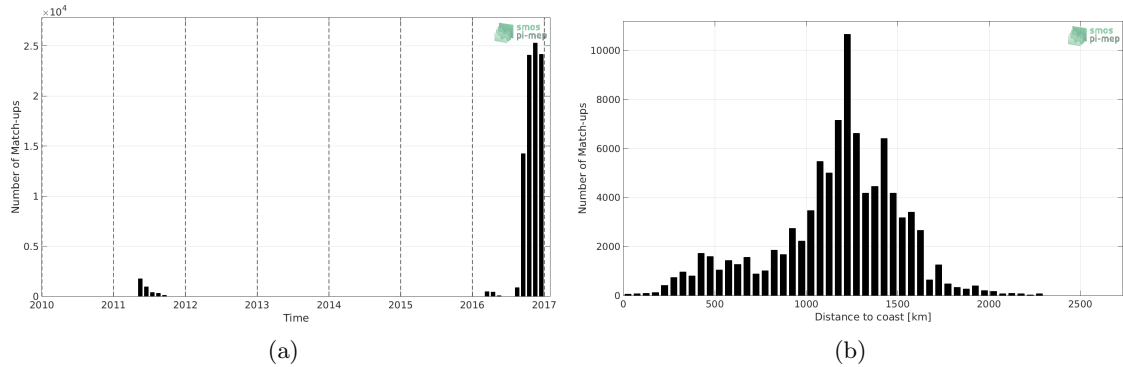
Figure 1: Number of match-ups between Surface drifters and SMOS-L3-BEC-OA-V1-9DAYS-0.25DEG SSS as a function of time (a) and as function of the distance to coast (b) over the North Pacific Ocean Pi-MEP region and for the full satellite product period.
