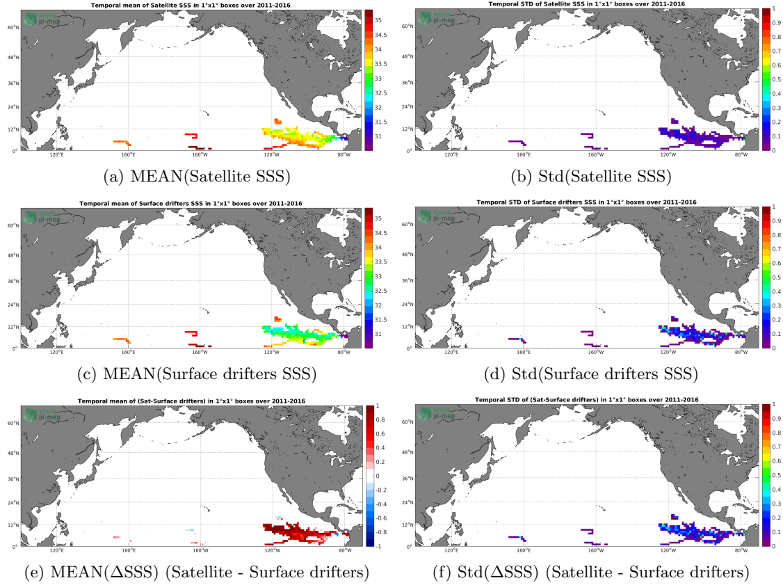
Figure 5: Temporal mean (left) and Std (right) of SSS from SMOS-L3-BEC-OA-V1-9DAYS-0.25DEG (top), Surface drifters (middle), and of \Delta SSS (Satellite - Surface drifters). Only match-up pairs are used to generate these maps.
