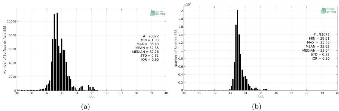
Figure 2: Histograms of SSS from Surface drifters (a) and SMOS-L3-BEC-OA-V1-9DAYS-0.25DEG (b) considering all match-up pairs per bins of 0.1 over the North Pacific Ocean Pi-MEP region and for the full satellite product period.
