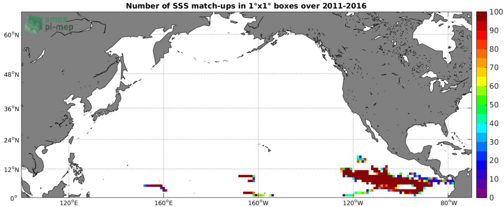
Figure 3: Number of SSS match-ups between Surface drifters SSS and the SMOS-L3-BEC-OA-V1-9DAYS-0.25DEG SSS product for the North Pacific Ocean Pi-MEP region over 1^\circ \times 1^\circ boxes and for the full satellite product period.
