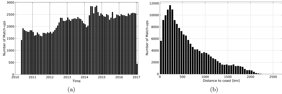
Figure 1: Number of match-ups between Argo and SMOS-L3-BEC-OA-V1-9DAYS-0.25DEG SSS as a function of time (a) and as function of the distance to coast (b) over the North Pacific Ocean Pi-MEP region and for the full satellite product period.
