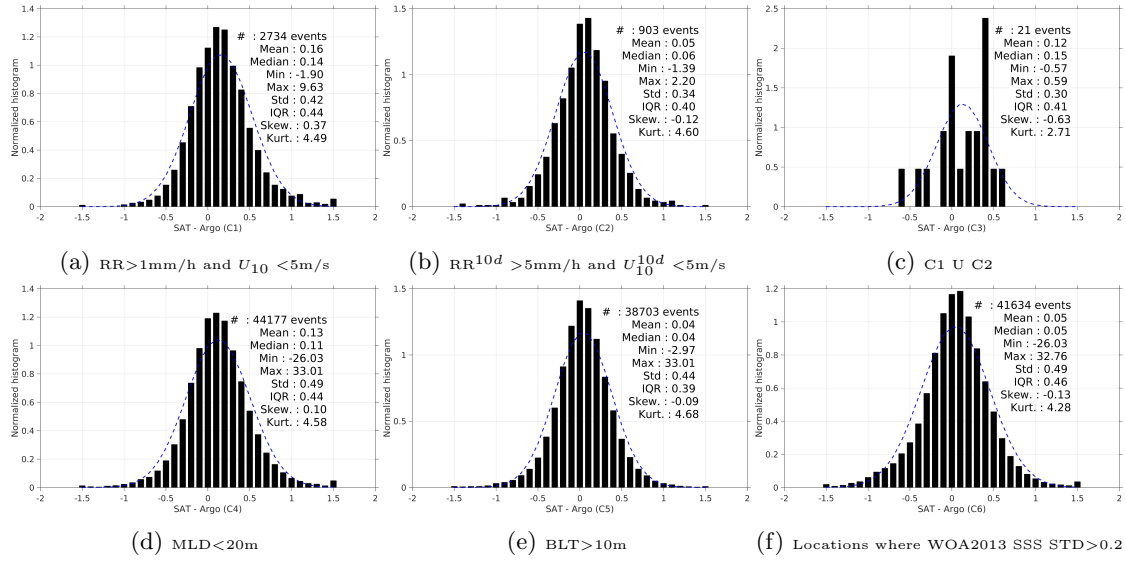
Figure 13: Normalized histogram of \Delta SSS (SMOS-L3-BEC-OA-V1-9DAYS-0.25DEG - Argo) for 6 different subdatasets corresponding to: RR>1mm/h and U_{10} <5m/s (a), RR 10d >5mm/h and U_{10}^{10d} <5m/s (b), C1 U C2 (c),MLD<20m (d),BLT>10m (e),Locations where WOA2013 SSS STD>0.2 (f).
