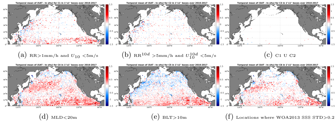
Figure 12: Temporal mean gridded over spatial boxes of size 1^\circ \times 1^\circ of \Delta SSS (SMOS-L3-BEC-OA-V1-9DAYS-0.25DEG - Argo) for 6 different subdatasets corresponding to: RR > 1\text{mm/h} and U_{10} < 5\text{m/s} (a), RR^{10d} > 5\text{mm/h} and U_{10}^{10d} < 5\text{m/s} (b), C1 U C2 (c), MLD < 20\text{m} (d), BLT > 10\text{m} (e), Locations where WOA2013 SSS STD > 0.2 (f).
