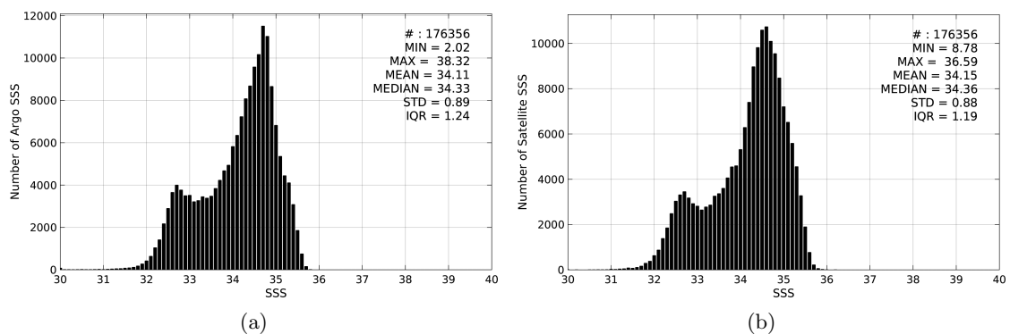
Figure 2: Histograms of SSS from Argo (a) and SMOS-L3-BEC-OA-V1-9DAYS-0.25DEG (b) considering all match-up pairs per bins of 0.1 over the North Pacific Ocean Pi-MEP region and for the full satellite product period.
