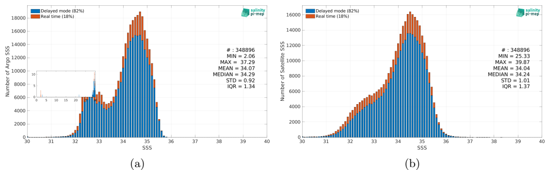
Figure 2: Histograms of SSS from Argo (a) and SMOS SSS L2-AVERAGED v700 (ESA) (b) considering all match-up pairs per bins of 0.1 over the North Pacific Ocean Pi-MEP region and for the full satellite product period.
