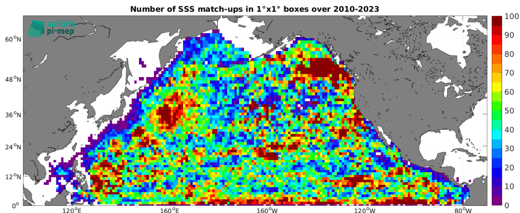
Figure 4: Number of SSS match-ups between Argo SSS and the SMOS SSS L2-AVERAGED v700 (ESA) SSS product for the North Pacific Ocean Pi-MEP region over 1^\circ \times 1^\circ boxes and for the full satellite product period.
