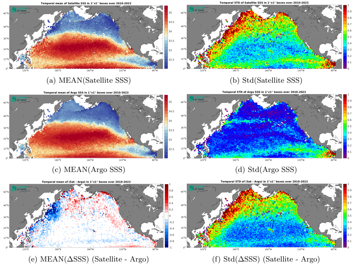
Figure 6: Temporal mean (left) and Std (right) of SSS from SMOS SSS L2-AVERAGED v700 (ESA) (top), Argo (middle), and of \Delta SSS (Satellite - Argo). Only match-up pairs are used to generate these maps.
