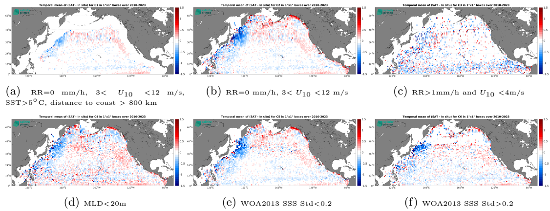
Figure 12: Temporal mean gridded over spatial boxes of size 1^\circ \times 1^\circ of \Delta SSS (SMOS SSS L2-AVERAGED v700 (ESA) - Argo) for 6 different subdatasets corresponding to:RR=0 mm/h, 3 < U_{10} < 12 m/s, SST >5^\circ\text{C} , distance to coast > 800 km (a), RR=0 mm/h, 3 < U_{10} < 12 m/s (b), RR >1 mm/h and U_{10} < 4 m/s (c),MLD <20 m (d),WOA2013 SSS Std <0.2 (e),WOA2013 SSS Std >0.2 (f).
