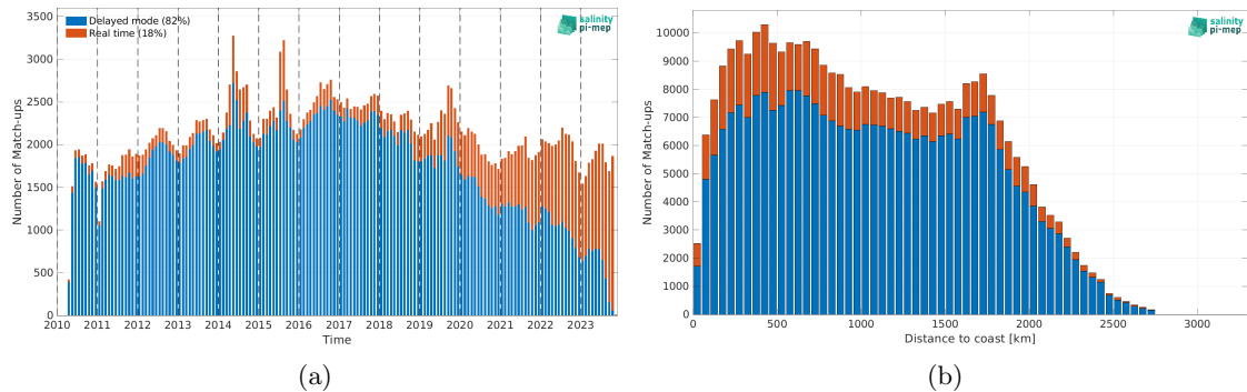
Figure 1: Number of match-ups between Argo and SMOS SSS L2-AVERAGED v700 (ESA) SSS as a function of time (a) and as function of the distance to coast (b) over the North Pacific Ocean Pi-MEP region and for the full satellite product period.
