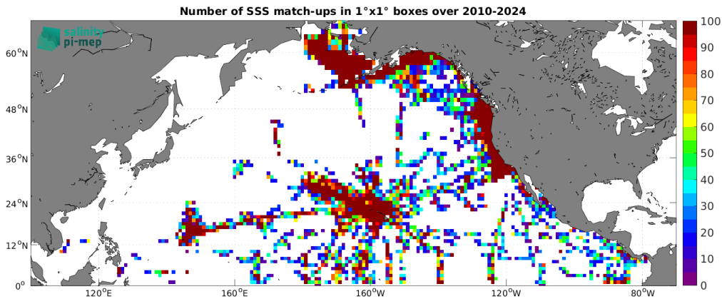
Figure 5: Number of SSS match-ups between TSG (SAMOS) SSS and the SMOS SSS L2 v700 (ESA) SSS product for the North Pacific Ocean Pi-MEP region over 1^\circ \times 1^\circ boxes and for the full satellite product period.
