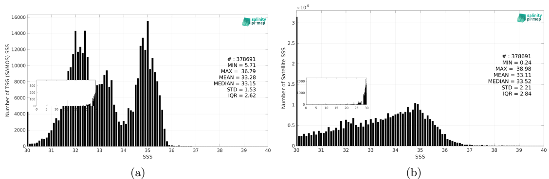
Figure 3: Histograms of SSS from TSG (SAMOS) (a) and SMOS SSS L2 v700 (ESA) (b) considering all match-up pairs per bins of 0.1 over the North Pacific Ocean Pi-MEP region and for the full satellite product period.
