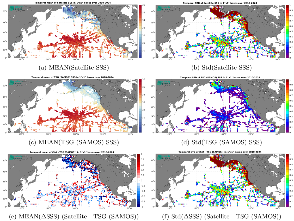
Figure 7: Temporal mean (left) and Std (right) of SSS from SMOS SSS L2 v700 (ESA) (top), TSG (SAMOS) (middle), and of \Delta SSS (Satellite - TSG (SAMOS)). Only match-up pairs are used to generate these maps.
