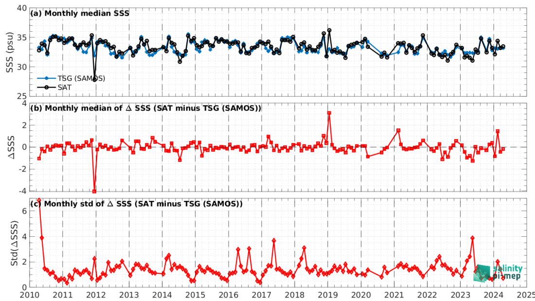
Figure 8: Time series of the monthly median SSS (top), median of \Delta SSS (Satellite - TSG (SAMOS)) and Std of \Delta SSS (Satellite - TSG (SAMOS)) over the North Pacific Ocean Pi-MEP region considering all match-ups collected by the Pi-MEP.
