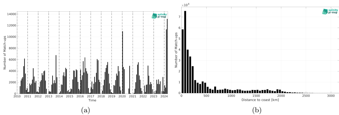
Figure 2: Number of match-ups between TSG (SAMOS) and SMOS SSS L2 v700 (ESA) SSS as a function of time (a) and as function of the distance to coast (b) over the North Pacific Ocean Pi-MEP region and for the full satellite product period.
