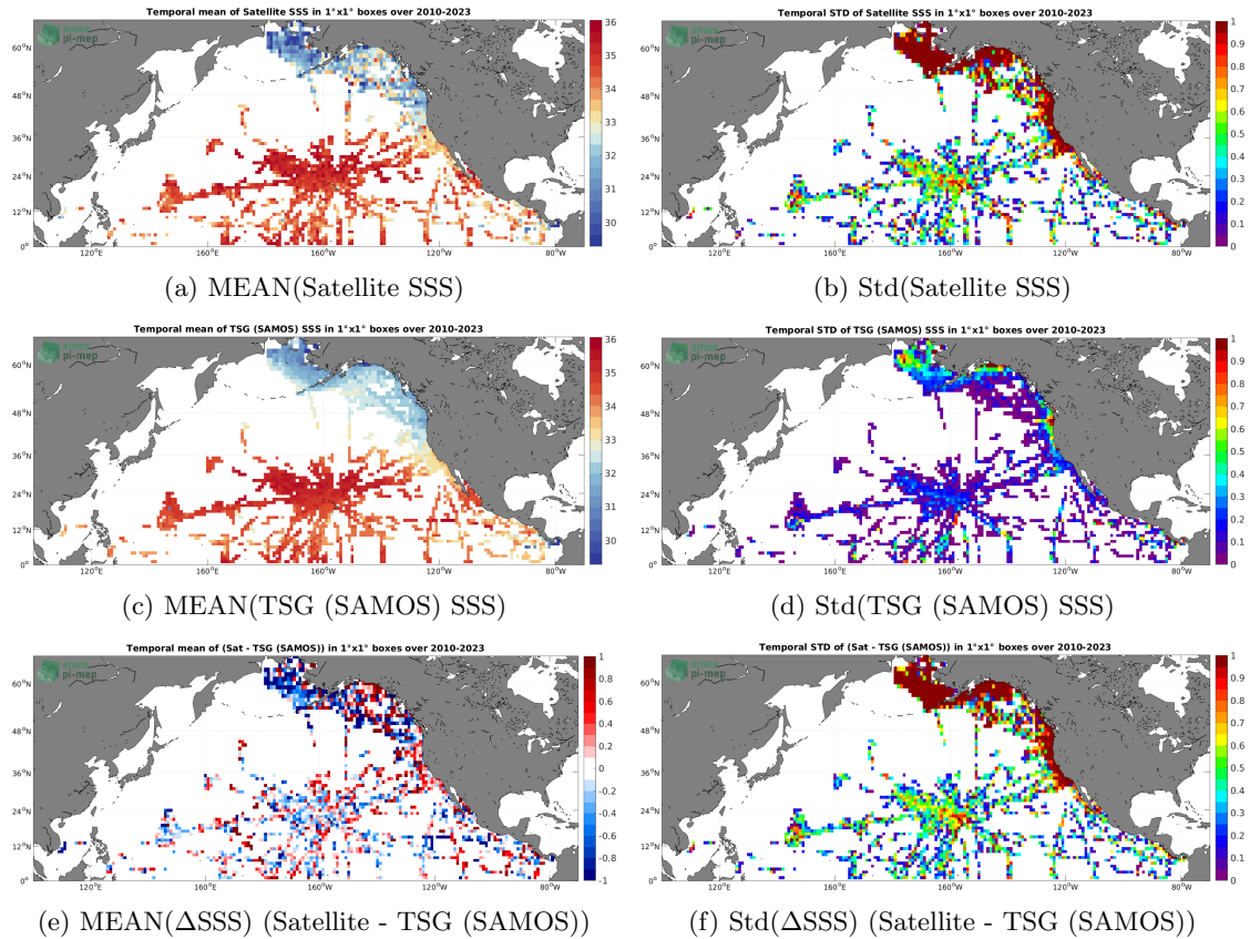
Figure 6: Temporal mean (left) and Std (right) of SSS from SMOS SSS L2 v700 (ESA) (top), TSG (SAMOS) (middle), and of \Delta SSS (Satellite - TSG (SAMOS)). Only match-up pairs are used to generate these maps.
