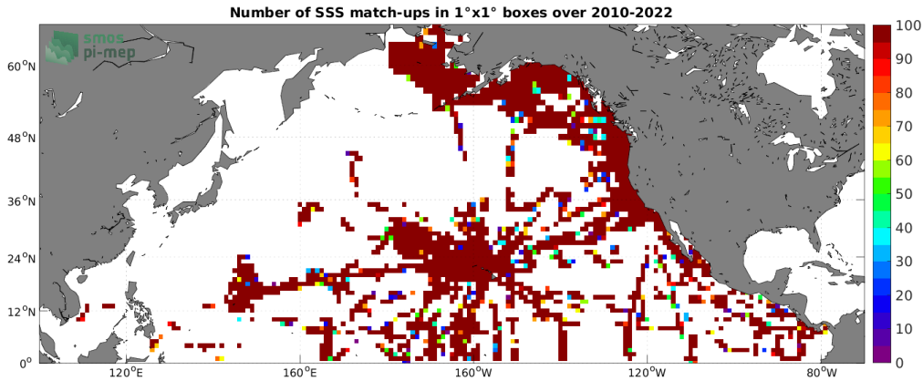
Figure 4: Number of SSS match-ups between TSG (SAMOS) SSS and the SMOS SSS L2 v700 (ESA) SSS product for the North Pacific Ocean Pi-MEP region over 1^\circ \times 1^\circ boxes and for the full satellite product period.
