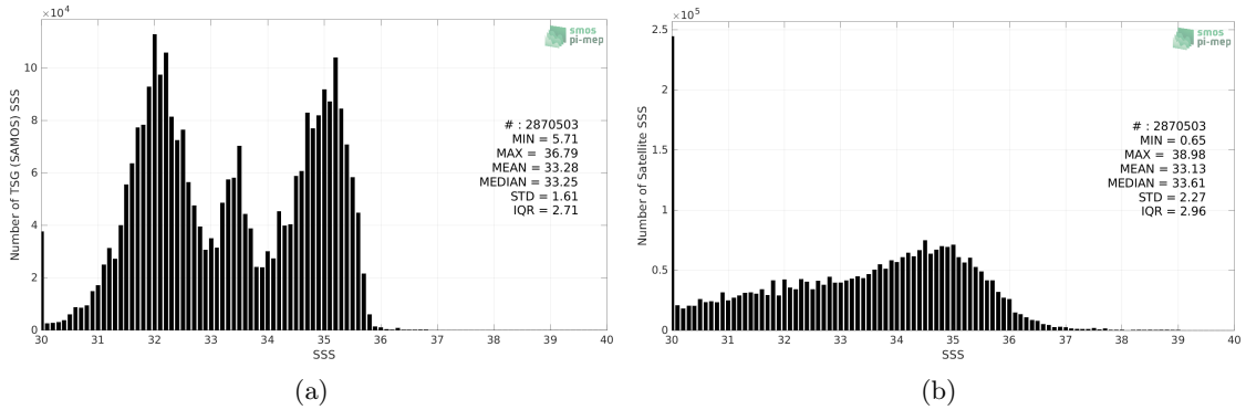
Figure 2: Histograms of SSS from TSG (SAMOS) (a) and SMOS SSS L2 v700 (ESA) (b) considering all match-up pairs per bins of 0.1 over the North Pacific Ocean Pi-MEP region and for the full satellite product period.
