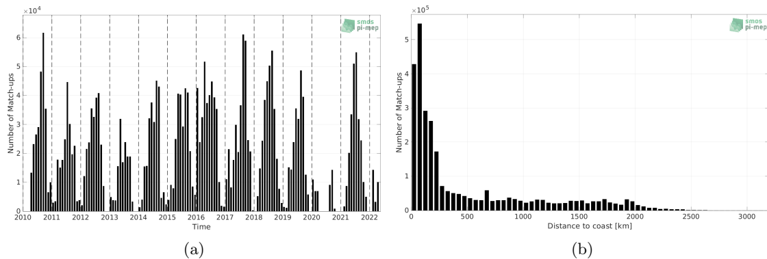
Figure 1: Number of match-ups between TSG (SAMOS) and SMOS SSS L2 v700 (ESA) SSS as a function of time (a) and as function of the distance to coast (b) over the North Pacific Ocean Pi-MEP region and for the full satellite product period.
