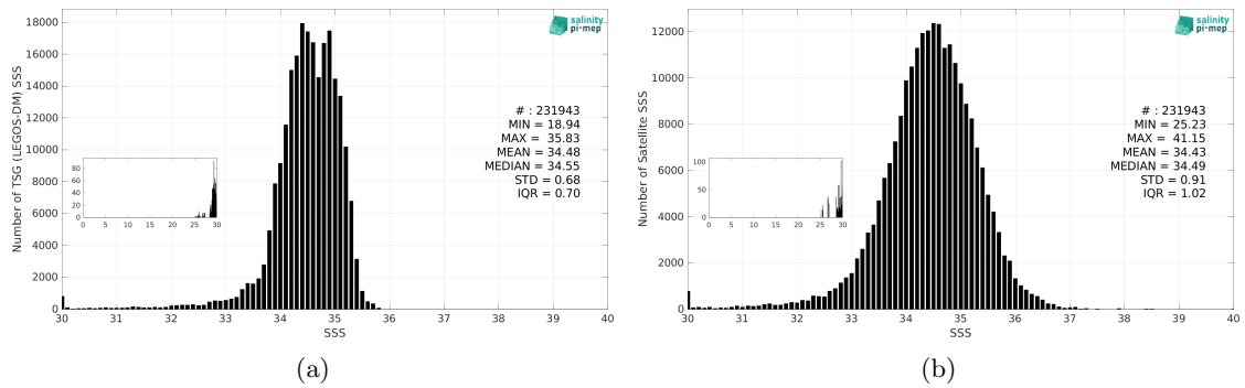
Figure 3: Histograms of SSS from TSG (LEGOS-DM) (a) and SMOS SSS L2 v700 (ESA) (b) considering all match-up pairs per bins of 0.1 over the North Pacific Ocean Pi-MEP region and for the full satellite product period.
