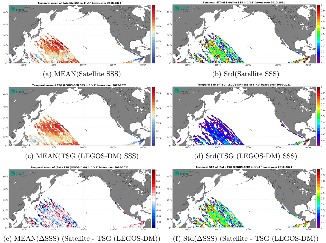
Figure 6: Temporal mean (left) and Std (right) of SSS from SMOS SSS L2 v700 (ESA) (top), TSG (LEGOS-DM) (middle), and of \Delta SSS (Satellite - TSG (LEGOS-DM)). Only match-up pairs are used to generate these maps.
