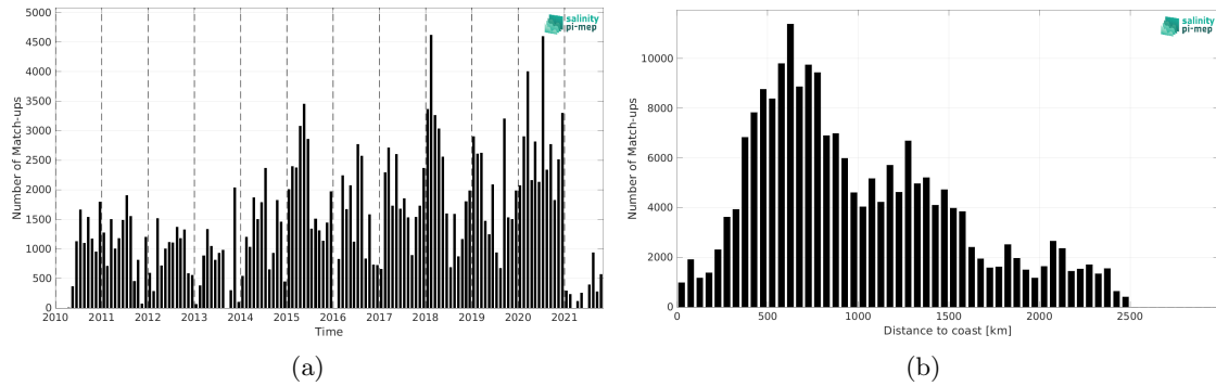
Figure 1: Number of match-ups between TSG (LEGOS-DM) and SMOS SSS L2 v700 (ESA) SSS as a function of time (a) and as function of the distance to the coast (b) over the North Pacific Ocean Pi-MEP region and for the full satellite product period.
