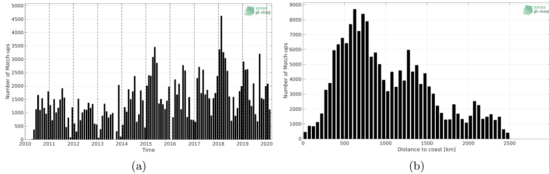
Figure 1: Number of match-ups between TSG (LEGOS-DM) and SMOS SSS L2 v700 (ESA) SSS as a function of time (a) and as function of the distance to coast (b) over the North Pacific Ocean Pi-MEP region and for the full satellite product period.
