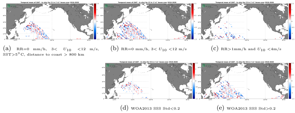
Figure 12: Temporal mean gridded over spatial boxes of size 1^\circ \times 1^\circ of \Delta SSS (SMOS SSS L2 v700 (ESA) - TSG (LEGOS-DM)) for 5 different subdatasets corresponding to: RR=0 mm/h, 3 < U_{10} < 12 m/s, SST >5^\circ\text{C} , distance to coast > 800 km (a), RR=0 mm/h, 3 < U_{10} < 12 m/s (b), RR >1 mm/h and U_{10} < 4 m/s (c), WOA2013 SSS Std <0.2 (d), WOA2013 SSS Std >0.2 (e).
