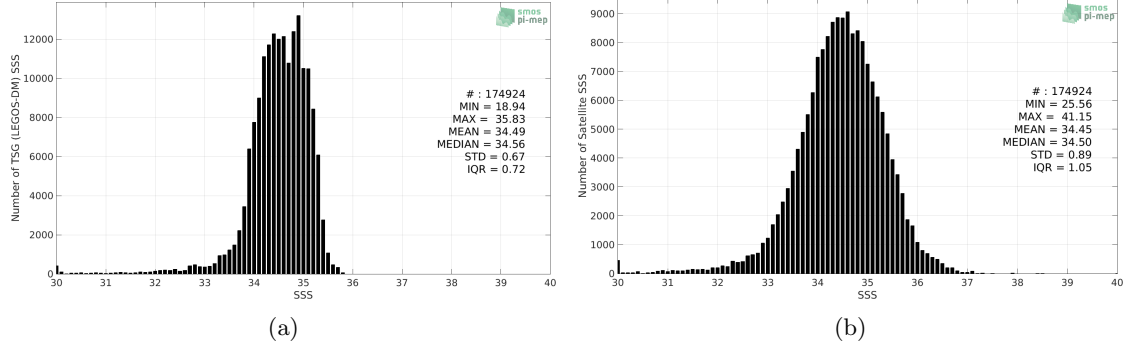
Figure 2: Histograms of SSS from TSG (LEGOS-DM) (a) and SMOS SSS L2 v700 (ESA) (b) considering all match-up pairs per bins of 0.1 over the North Pacific Ocean Pi-MEP region and for the full satellite product period.
