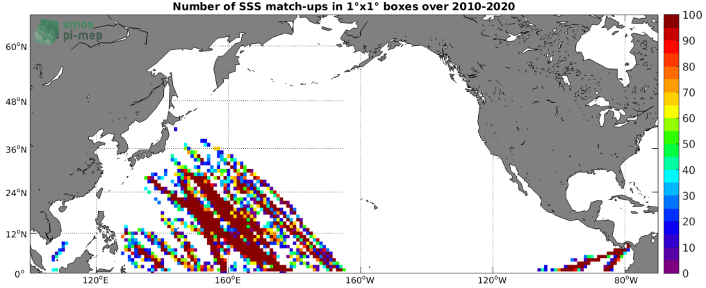
Figure 4: Number of SSS match-ups between TSG (LEGOS-DM) SSS and the SMOS SSS L2 v700 (ESA) SSS product for the North Pacific Ocean Pi-MEP region over 1^\circ \times 1^\circ boxes and for the full satellite product period.
