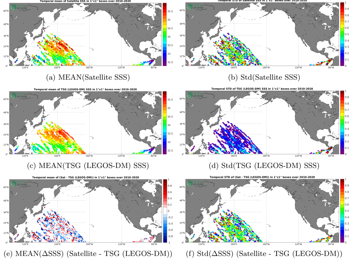
Figure 6: Temporal mean (left) and Std (right) of SSS from SMOS SSS L2 v700 (ESA) (top), TSG (LEGOS-DM) (middle), and of \Delta\text{SSS} (Satellite - TSG (LEGOS-DM)). Only match-up pairs are used to generate these maps.
