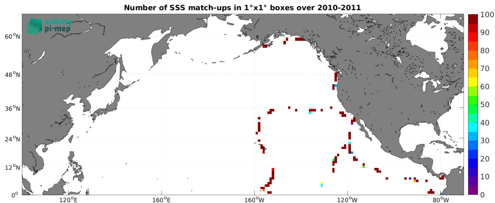
Figure 5: Number of SSS match-ups between TSG (GOSUD-Sailing-ship) SSS and the SMOS SSS L2 v700 (ESA) SSS product for the North Pacific Ocean Pi-MEP region over 1^\circ \times 1^\circ boxes and for the full satellite product period.
