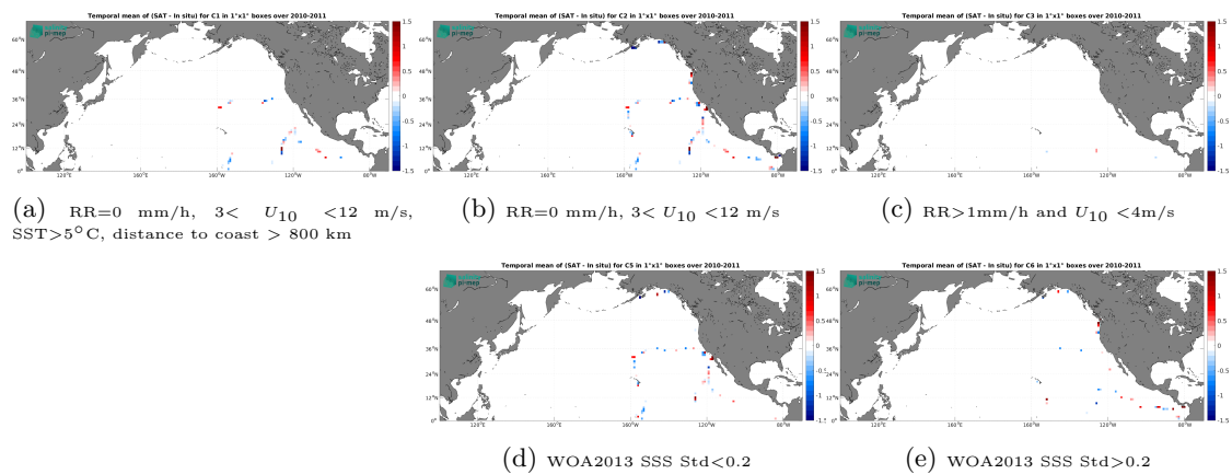
Figure 14: Temporal mean gridded over spatial boxes of size 1^\circ \times 1^\circ of \Delta SSS (SMOS SSS L2 v700 (ESA) - TSG (GOSUD-Sailing-ship)) for 5 different subdatasets corresponding to: RR=0 mm/h, 3 < U_{10} < 12 m/s, SST > 5^\circ C , distance to coast > 800 km (a), RR=0 mm/h, 3 < U_{10} < 12 m/s (b), RR > 1mm/h and U_{10} < 4 m/s (c), WOA2013 SSS Std < 0.2 (d), WOA2013 SSS Std > 0.2 (e).
