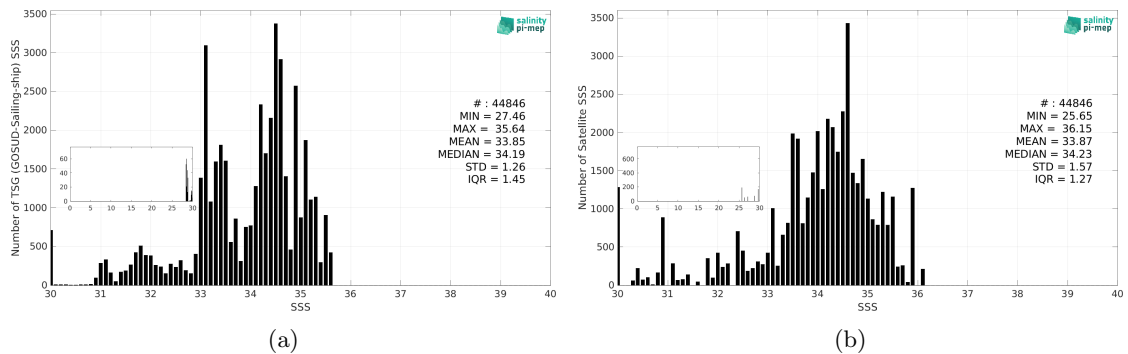
Figure 3: Histograms of SSS from TSG (GOSUD-Sailing-ship) (a) and SMOS SSS L2 v700 (ESA) (b) considering all match-up pairs per bins of 0.1 over the North Pacific Ocean Pi-MEP region and for the full satellite product period.
