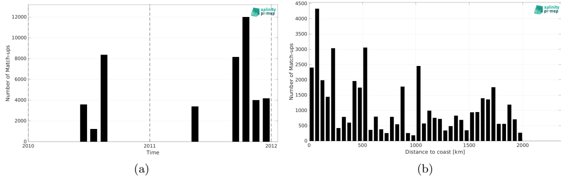
Figure 2: Number of match-ups between TSG (GOSUD-Sailing-ship) and SMOS SSS L2 v700 (ESA) SSS as a function of time (a) and as function of the distance to coast (b) over the North Pacific Ocean Pi-MEP region and for the full satellite product period.
