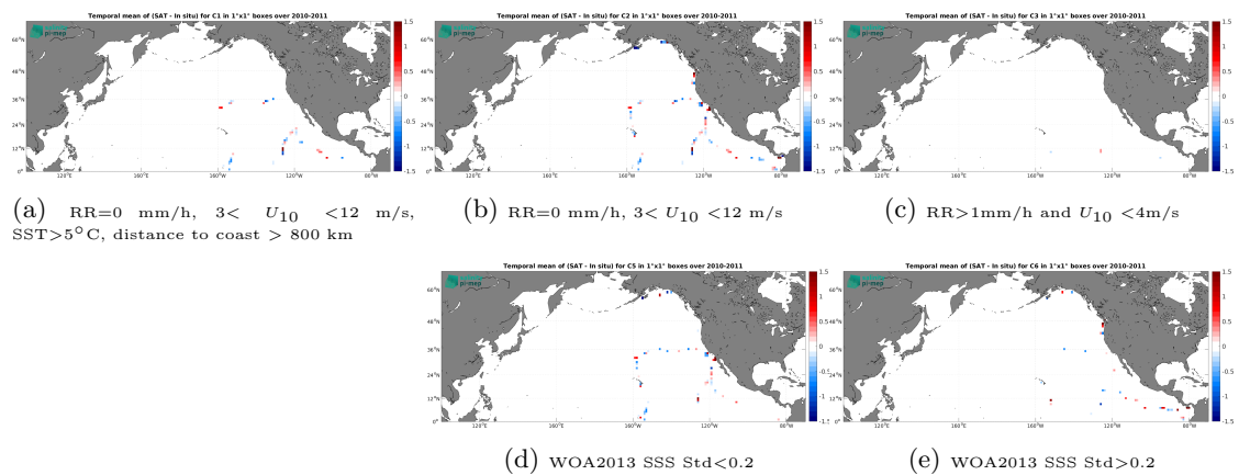
Figure 14: Temporal mean gridded over spatial boxes of size 1^\circ \times 1^\circ of \Delta SSS (SMOS SSS L2 v700 (ESA) - TSG (GOSUD-Sailing-ship)) for 5 different subdatasets corresponding to:RR=0 mm/h, 3 < U_{10} < 12 m/s, SST>5°C, distance to coast > 800 km (a), RR=0 mm/h, 3 < U_{10} < 12 m/s (b), RR>1mm/h and U_{10} < 4 m/s (c), WOA2013 SSS Std<0.2 (d), WOA2013 SSS Std>0.2 (e).
