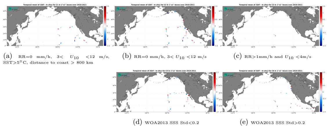
Figure 12: Temporal mean gridded over spatial boxes of size 1^\circ \times 1^\circ of \Delta\text{SSS} (SMOS SSS L2 v700 (ESA) - TSG (GOSUD-Sailing-ship)) for 5 different subdatasets corresponding to:RR=0 mm/h, 3 < U_{10} < 12 m/s, SST>5°C, distance to coast > 800 km (a), RR=0 mm/h, 3 < U_{10} < 12 m/s (b), RR>1mm/h and U_{10} < 4 m/s (c), WOA2013 SSS Std<0.2 (d), WOA2013 SSS Std>0.2 (e).
