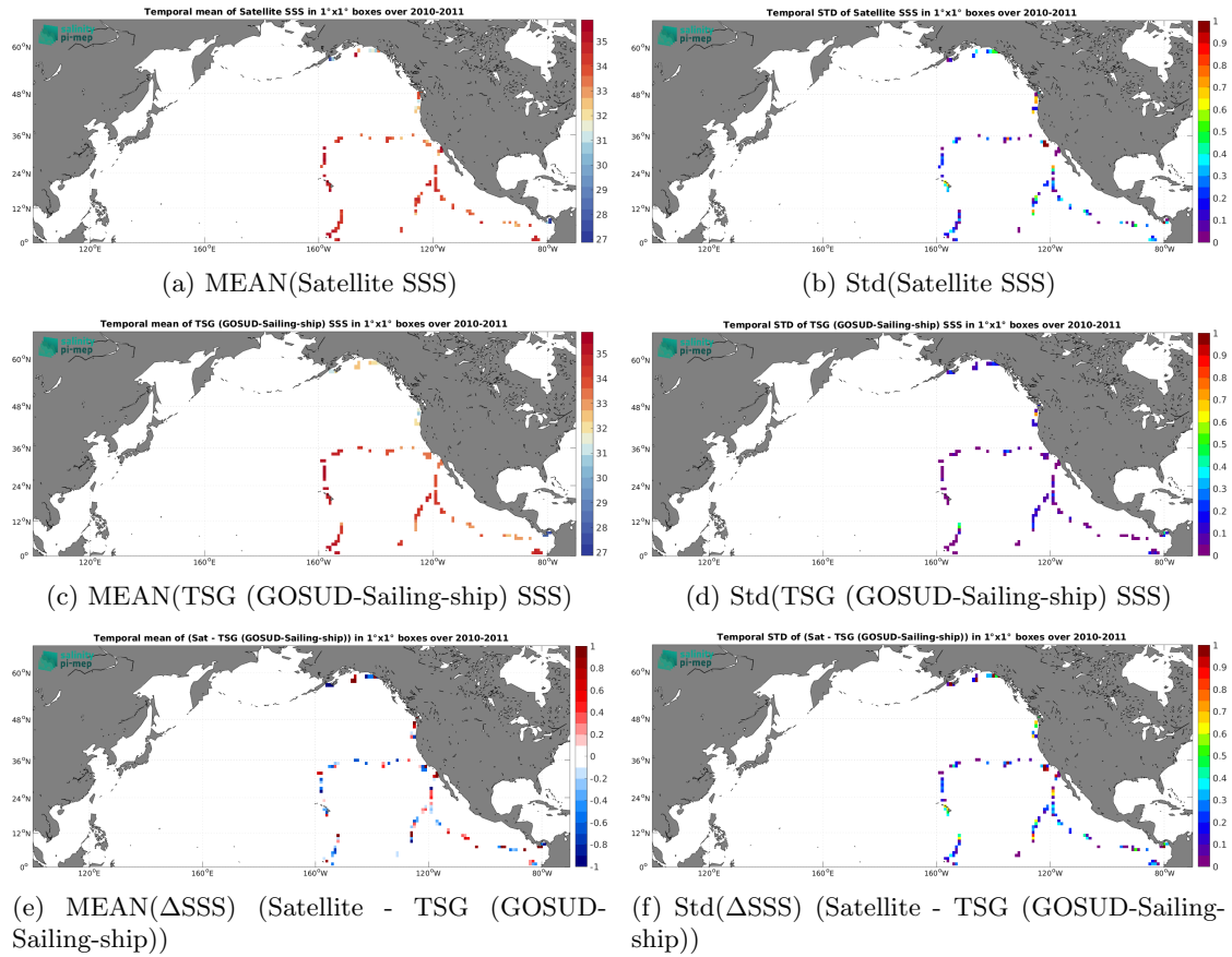
Figure 6: Temporal mean (left) and Std (right) of SSS from SMOS SSS L2 v700 (ESA) (top), TSG (GOSUD-Sailing-ship) (middle), and of \Delta SSS (Satellite - TSG (GOSUD-Sailing-ship)). Only match-up pairs are used to generate these maps.
