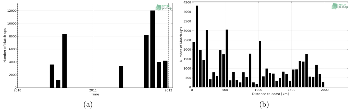
Figure 1: Number of match-ups between TSG (GOSUD-Sailing-ship) and SMOS SSS L2 v700 (ESA) SSS as a function of time (a) and as function of the distance to coast (b) over the North Pacific Ocean Pi-MEP region and for the full satellite product period.
