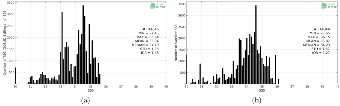
Figure 2: Histograms of SSS from TSG (GOSUD-Sailing-ship) (a) and SMOS SSS L2 v700 (ESA) (b) considering all match-up pairs per bins of 0.1 over the North Pacific Ocean Pi-MEP region and for the full satellite product period.
