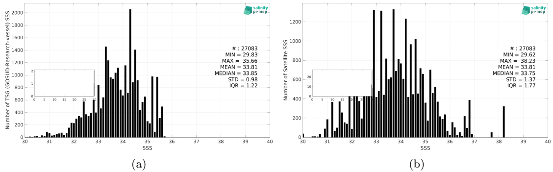
Figure 3: Histograms of SSS from TSG (GOSUD-Research-vessel) (a) and SMOS SSS L2 v700 (ESA) (b) considering all match-up pairs per bins of 0.1 over the North Pacific Ocean Pi-MEP region and for the full satellite product period.
