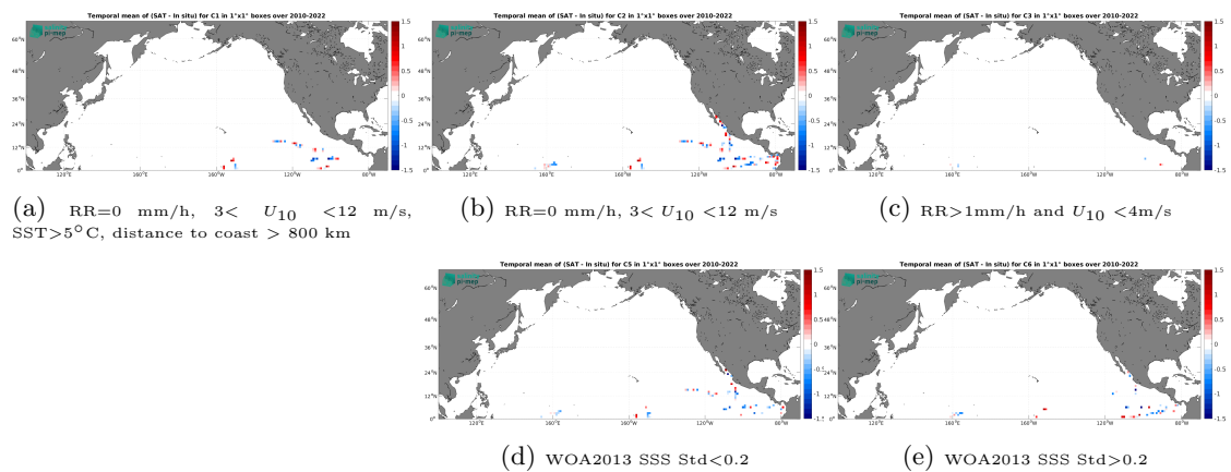
Figure 14: Temporal mean gridded over spatial boxes of size 1^\circ \times 1^\circ of \Delta\text{SSS} (SMOS SSS L2 v700 (ESA) - TSG (GOSUD-Research-vessel)) for 5 different subdatasets corresponding to: RR=0 mm/h, 3 < U_{10} < 12 m/s, SST > 5°C, distance to coast > 800 km (a), RR=0 mm/h, 3 < U_{10} < 12 m/s (b), RR > 1mm/h and U_{10} < 4 m/s (c), WOA2013 SSS Std < 0.2 (d), WOA2013 SSS Std > 0.2 (e).
