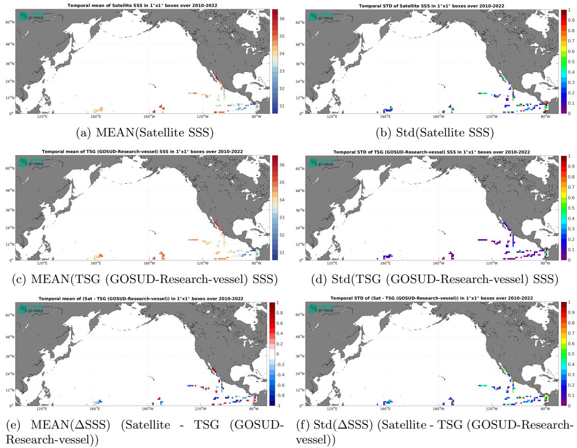
Figure 7: Temporal mean (left) and Std (right) of SSS from SMOS SSS L2 v700 (ESA) (top), TSG (GOSUD-Research-vessel) (middle), and of \Delta SSS (Satellite - TSG (GOSUD-Research-vessel)). Only match-up pairs are used to generate these maps.
