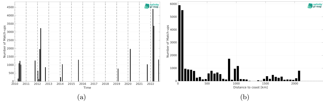
Figure 2: Number of match-ups between TSG (GOSUD-Research-vessel) and SMOS SSS L2 v700 (ESA) SSS as a function of time (a) and as function of the distance to coast (b) over the North Pacific Ocean Pi-MEP region and for the full satellite product period.
