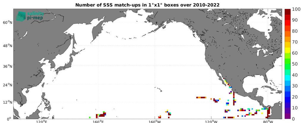
Figure 5: Number of SSS match-ups between TSG (GOSUD-Research-vessel) SSS and the SMOS SSS L2 v700 (ESA) SSS product for the North Pacific Ocean Pi-MEP region over 1^\circ \times 1^\circ boxes and for the full satellite product period.
