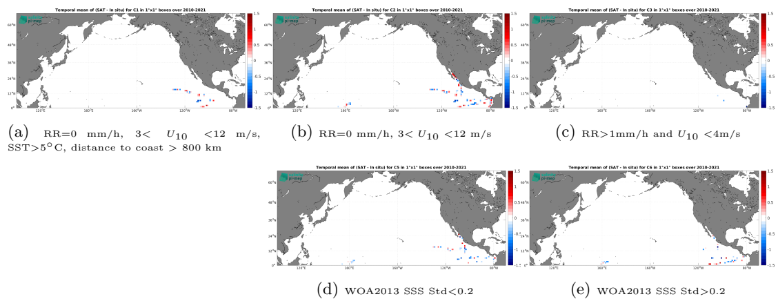
Figure 12: Temporal mean gridded over spatial boxes of size 1^\circ \times 1^\circ of \Delta\text{SSS} (SMOS SSS L2 v700 (ESA) - TSG (GOSUD-Research-vessel)) for 5 different subdatasets corresponding to: RR=0 mm/h, 3 < U_{10} < 12 m/s, SST > 5°C, distance to coast > 800 km (a), RR=0 mm/h, 3 < U_{10} < 12 m/s (b), RR > 1mm/h and U_{10} < 4 m/s (c), WOA2013 SSS Std < 0.2 (d), WOA2013 SSS Std > 0.2 (e).
