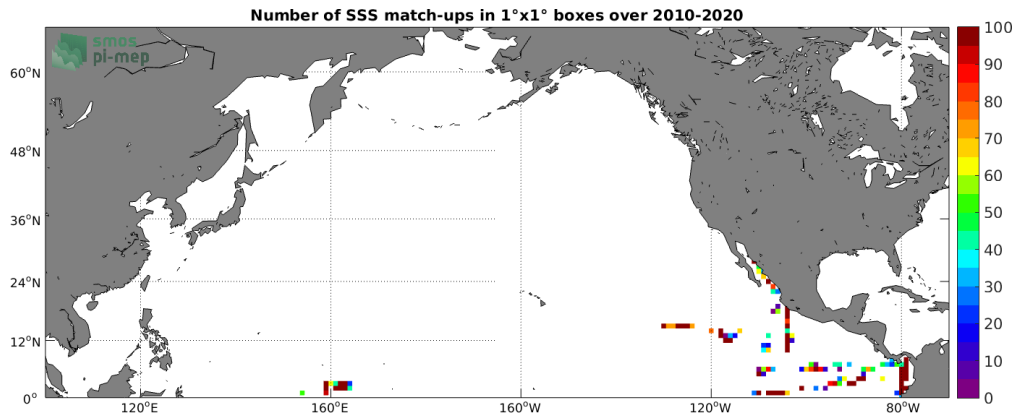
Figure 4: Number of SSS match-ups between TSG (GOSUD-Research-vessel) SSS and the SMOS SSS L2 v700 (ESA) SSS product for the North Pacific Ocean Pi-MEP region over 1^\circ \times 1^\circ boxes and for the full satellite product period.
