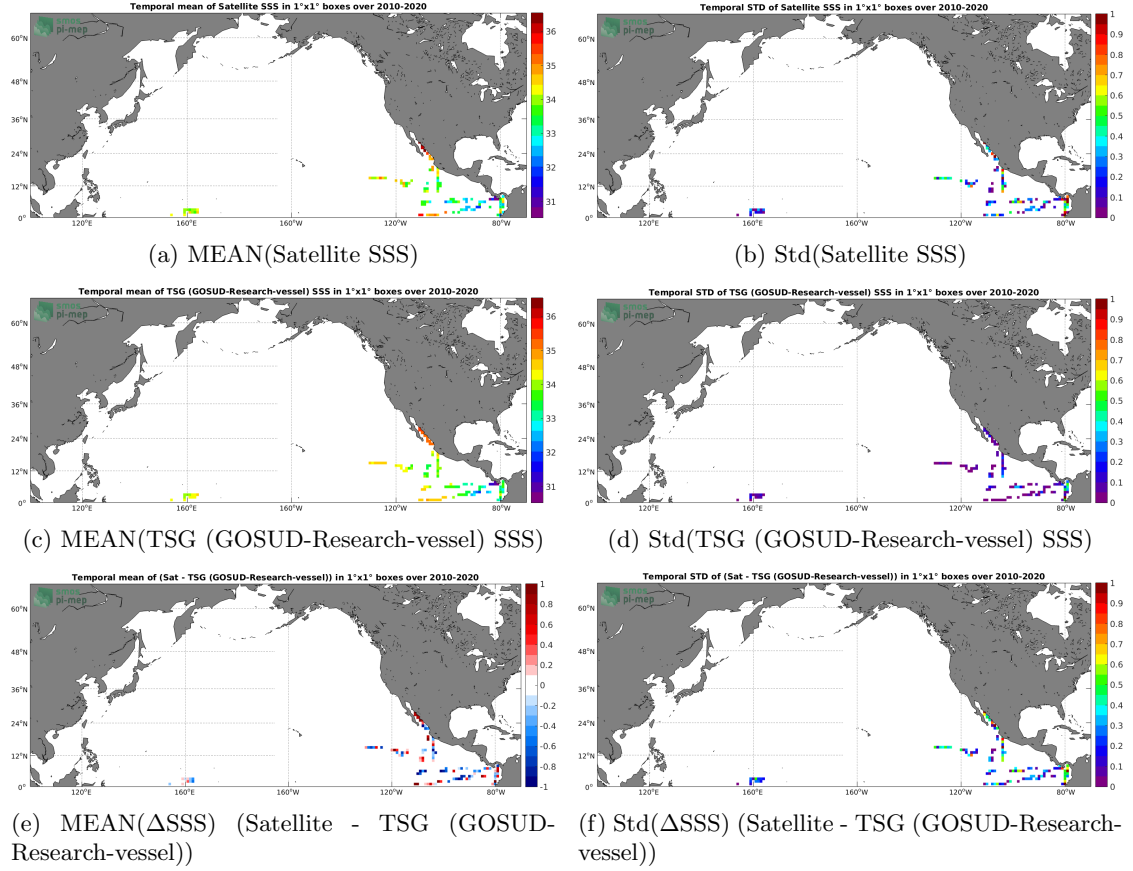
Figure 6: Temporal mean (left) and Std (right) of SSS from SMOS SSS L2 v700 (ESA) (top), TSG (GOSUD-Research-vessel) (middle), and of \Delta SSS (Satellite - TSG (GOSUD-Research-vessel)). Only match-up pairs are used to generate these maps.
