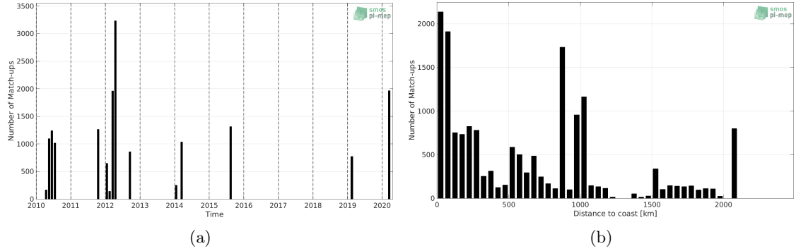
Figure 1: Number of match-ups between TSG (GOSUD-Research-vessel) and SMOS SSS L2 v700 (ESA) SSS as a function of time (a) and as function of the distance to coast (b) over the North Pacific Ocean Pi-MEP region and for the full satellite product period.
