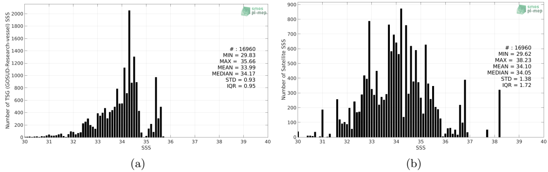
Figure 2: Histograms of SSS from TSG (GOSUD-Research-vessel) (a) and SMOS SSS L2 v700 (ESA) (b) considering all match-up pairs per bins of 0.1 over the North Pacific Ocean Pi-MEP region and for the full satellite product period.
