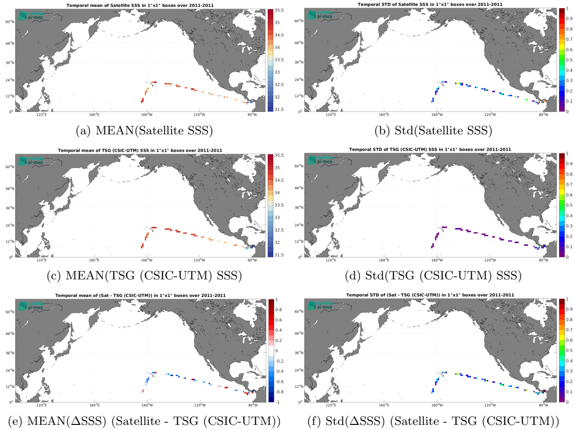
Figure 6: Temporal mean (left) and Std (right) of SSS from SMOS SSS L2 v700 (ESA) (top), TSG (CSIC-UTM) (middle), and of \Delta SSS (Satellite - TSG (CSIC-UTM)). Only match-up pairs are used to generate these maps.
