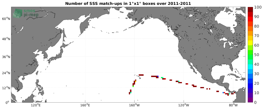
Figure 4: Number of SSS match-ups between TSG (CSIC-UTM) SSS and the SMOS SSS L2 v700 (ESA) SSS product for the North Pacific Ocean Pi-MEP region over 1^\circ \times 1^\circ boxes and for the full satellite product period.
