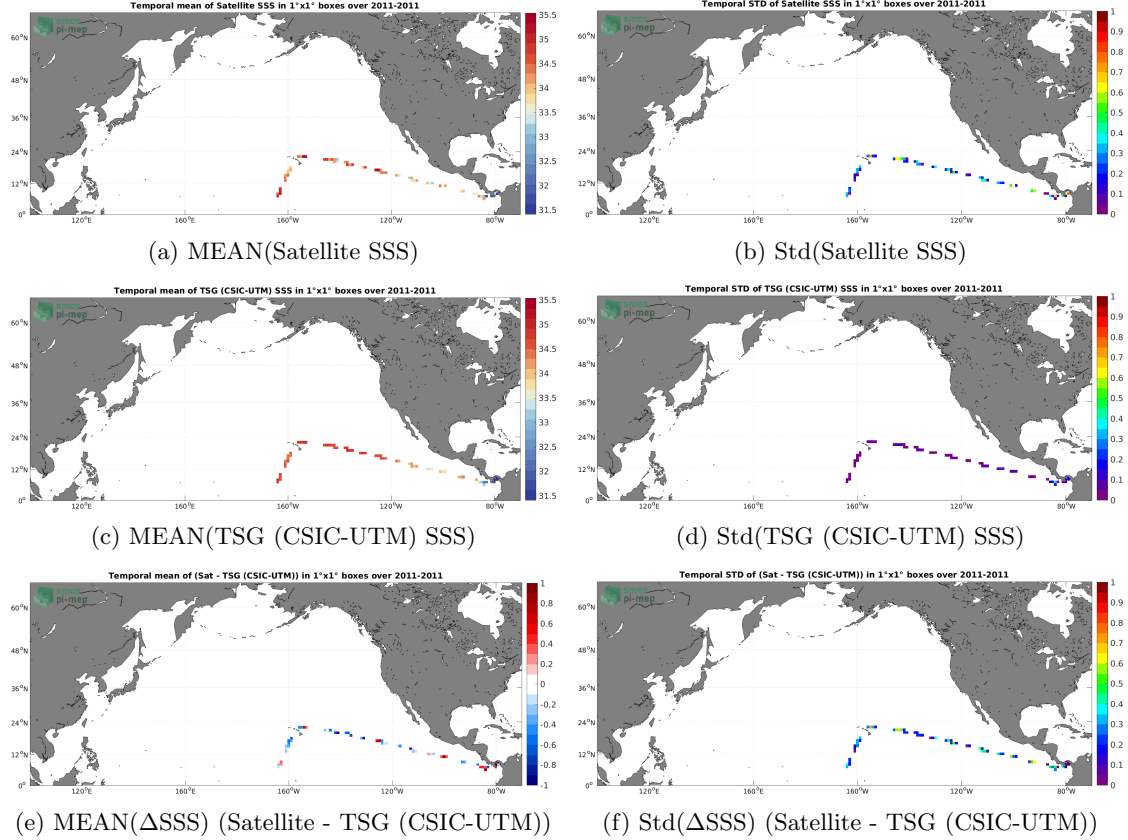
Figure 6: Temporal mean (left) and Std (right) of SSS from SMOS SSS L2 v700 (ESA) (top), TSG (CSIC-UTM) (middle), and of \Delta\text{SSS} (Satellite - TSG (CSIC-UTM)). Only match-up pairs are used to generate these maps.
