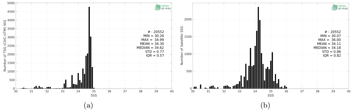
Figure 2: Histograms of SSS from TSG (CSIC-UTM) (a) and SMOS SSS L2 v700 (ESA) (b) considering all match-up pairs per bins of 0.1 over the North Pacific Ocean Pi-MEP region and for the full satellite product period.
