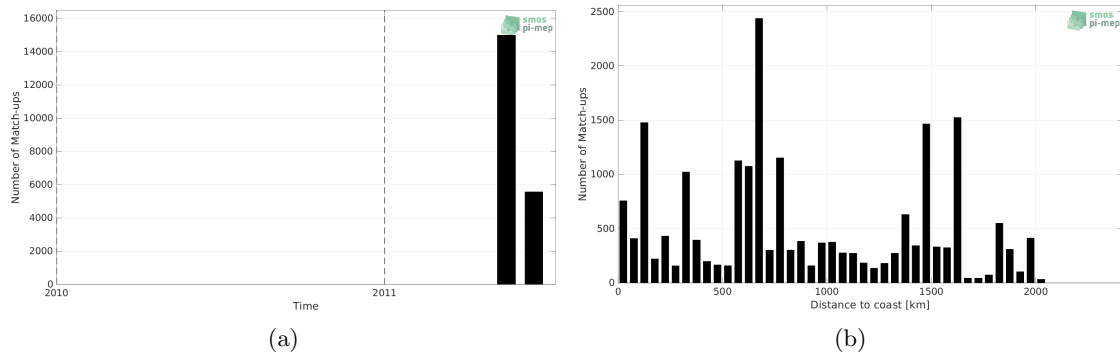
Figure 1: Number of match-ups between TSG (CSIC-UTM) and SMOS SSS L2 v700 (ESA) SSS as a function of time (a) and as function of the distance to coast (b) over the North Pacific Ocean Pi-MEP region and for the full satellite product period.
