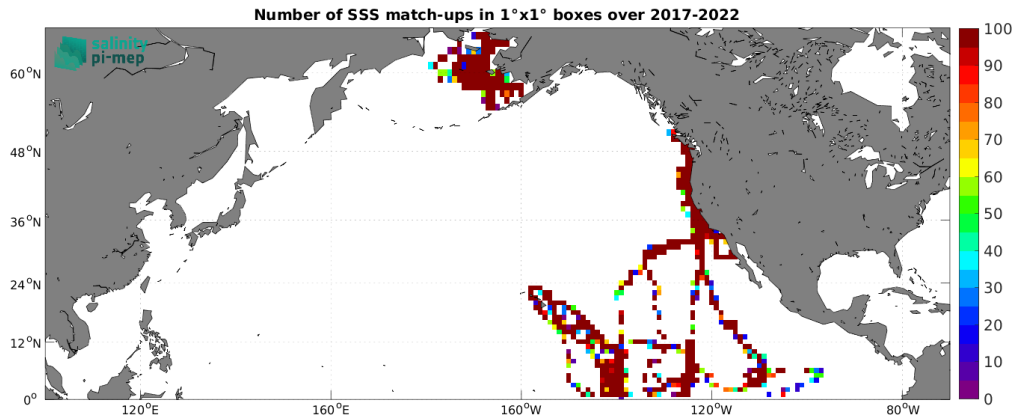
Figure 4: Number of SSS match-ups between Saildrone SSS and the SMOS SSS L2 v700 (ESA) SSS product for the North Pacific Ocean Pi-MEP region over 1^\circ \times 1^\circ boxes and for the full satellite product period.
