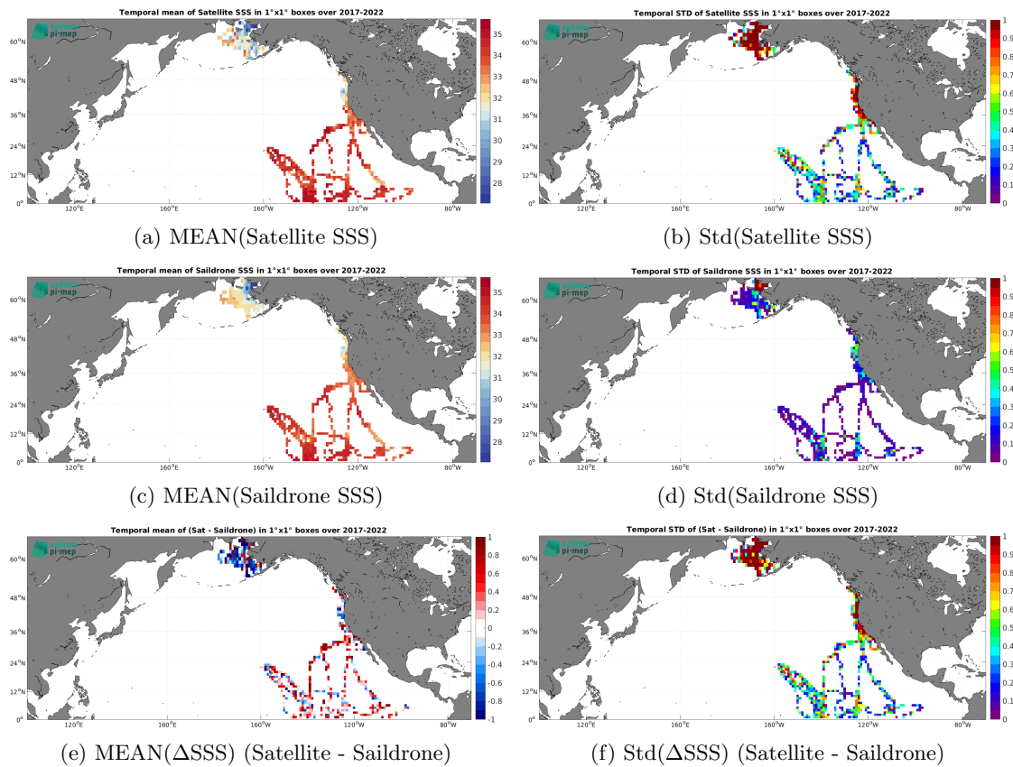
Figure 6: Temporal mean (left) and Std (right) of SSS from SMOS SSS L2 v700 (ESA) (top), Saildrone (middle), and of \Delta SSS (Satellite - Saildrone). Only match-up pairs are used to generate these maps.
