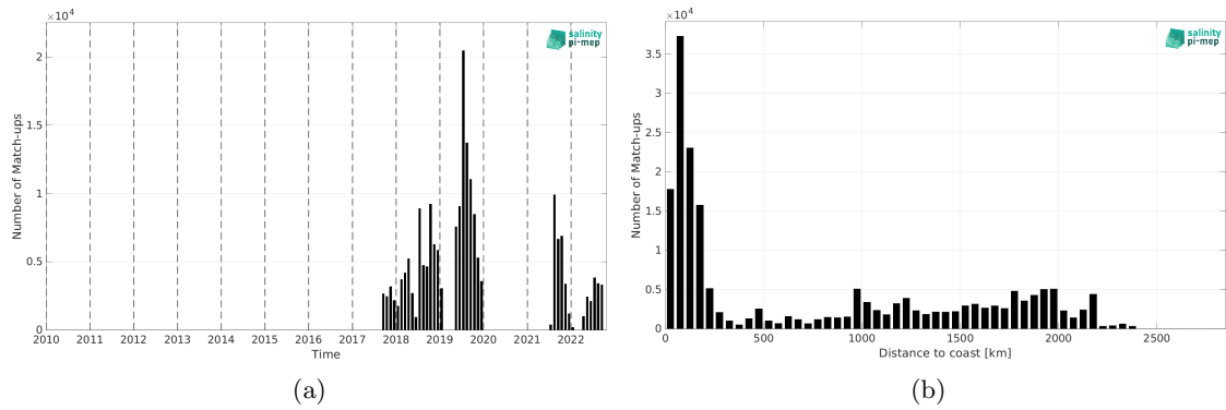
Figure 1: Number of match-ups between Saildrone and SMOS SSS L2 v700 (ESA) SSS as a function of time (a) and as function of the distance to coast (b) over the North Pacific Ocean Pi-MEP region and for the full satellite product period.
