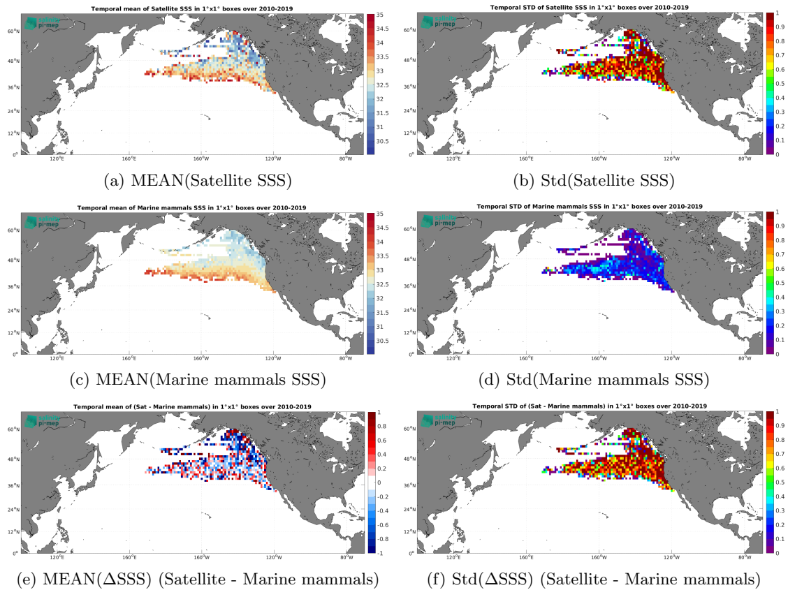
Figure 6: Temporal mean (left) and Std (right) of SSS from SMOS SSS L2 v700 (ESA) (top), Marine mammals (middle), and of \Delta SSS (Satellite - Marine mammals). Only match-up pairs are used to generate these maps.
