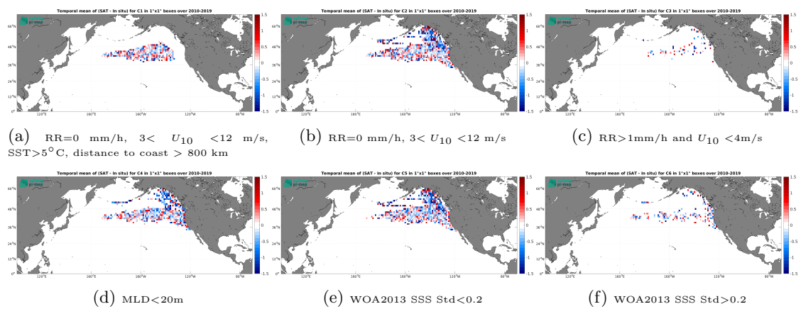
Figure 12: Temporal mean gridded over spatial boxes of size 1^\circ \times 1^\circ of \Delta SSS (SMOS SSS L2 v700 (ESA) - Marine mammals) for 6 different subdatasets corresponding to:RR=0 mm/h, 3 < U_{10} < 12 m/s, SST >5^\circ C, distance to coast > 800 km (a), RR=0 mm/h, 3 < U_{10} < 12 m/s (b), RR >1 mm/h and U_{10} < 4 m/s (c),MLD <20 m (d),WOA2013 SSS Std <0.2 (e),WOA2013 SSS Std >0.2 (f).
