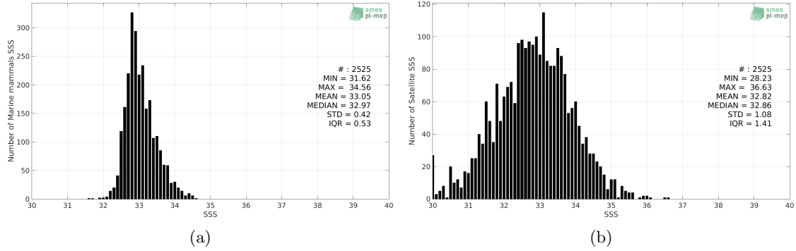
Figure 2: Histograms of SSS from Marine mammals (a) and SMOS SSS L2 v700 (ESA) (b) considering all match-up pairs per bins of 0.1 over the North Pacific Ocean Pi-MEP region and for the full satellite product period.
