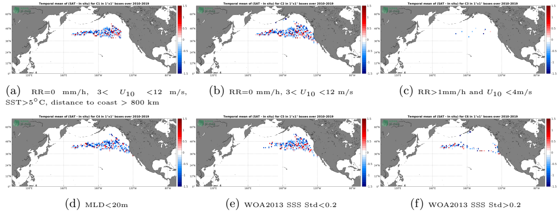
Figure 12: Temporal mean gridded over spatial boxes of size 1^\circ \times 1^\circ of \Delta SSS (SMOS SSS L2 v700 (ESA) - Marine mammals) for 6 different subdatasets corresponding to: RR=0 mm/h, 3 < U_{10} < 12 m/s, SST > 5^\circ C , distance to coast > 800 km (a), RR=0 mm/h, 3 < U_{10} < 12 m/s (b), RR > 1 mm/h and U_{10} < 4 m/s (c), MLD < 20 m (d), WOA2013 SSS Std < 0.2 (e), WOA2013 SSS Std > 0.2 (f).
