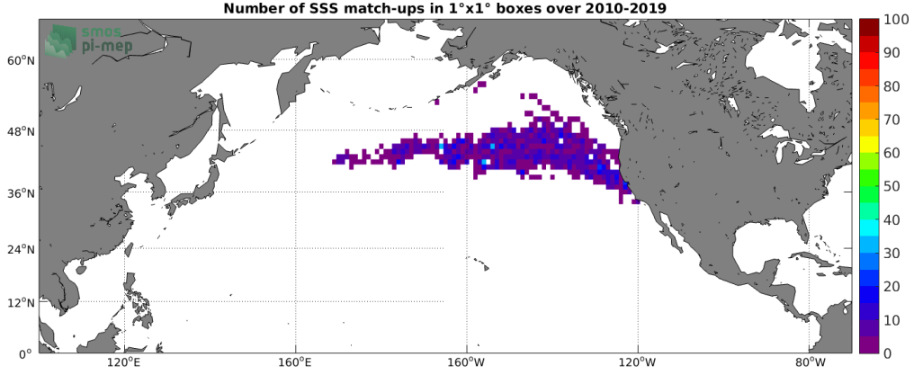
Figure 4: Number of SSS match-ups between Marine mammals SSS and the SMOS SSS L2 v700 (ESA) SSS product for the North Pacific Ocean Pi-MEP region over 1^\circ \times 1^\circ boxes and for the full satellite product period.
