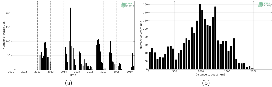
Figure 1: Number of match-ups between Marine mammals and SMOS SSS L2 v700 (ESA) SSS as a function of time (a) and as function of the distance to coast (b) over the North Pacific Ocean Pi-MEP region and for the full satellite product period.
