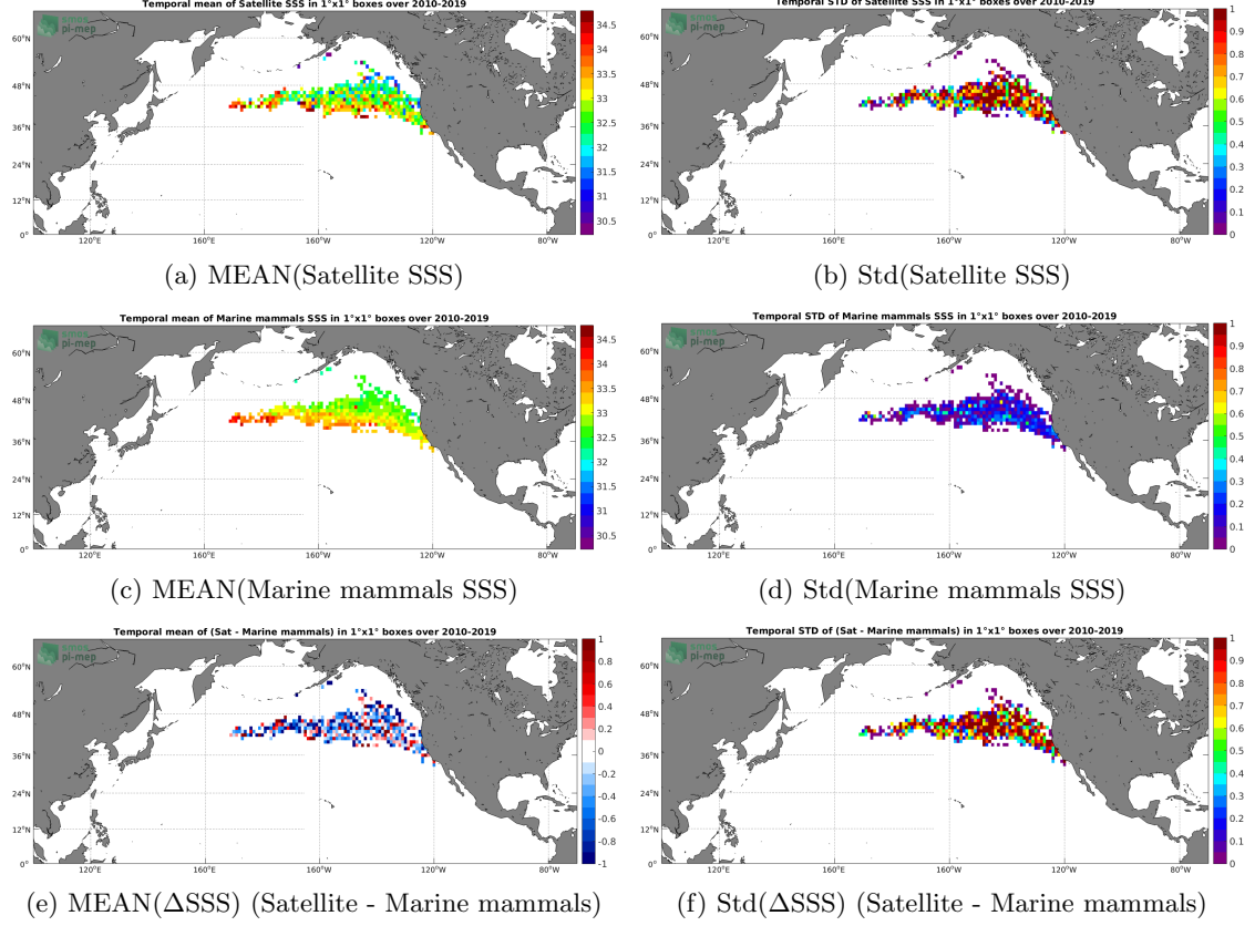
Figure 6: Temporal mean (left) and Std (right) of SSS from SMOS SSS L2 v700 (ESA) (top), Marine mammals (middle), and of \Delta\text{SSS} (Satellite - Marine mammals). Only match-up pairs are used to generate these maps.
