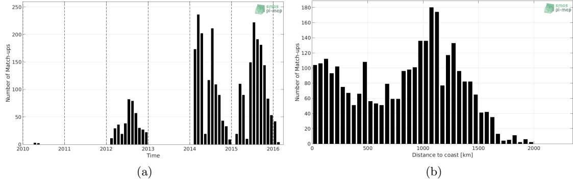
Figure 1: Number of match-ups between Sea mammals and SMOS SSS L2 v700 (ESA) SSS as a function of time (a) and as function of the distance to coast (b) over the North Pacific Ocean Pi-MEP region and for the full satellite product period.
