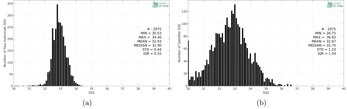
Figure 2: Histograms of SSS from Sea mammals (a) and SMOS SSS L2 v700 (ESA) (b) considering all match-up pairs per bins of 0.1 over the North Pacific Ocean Pi-MEP region and for the full satellite product period.
