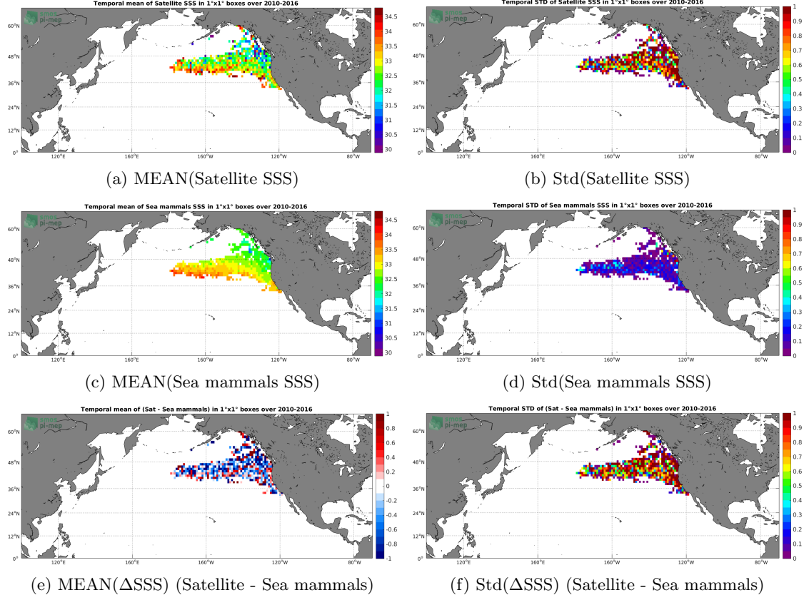
Figure 6: Temporal mean (left) and Std (right) of SSS from SMOS SSS L2 v700 (ESA) (top), Sea mammals (middle), and of \Delta SSS (Satellite - Sea mammals). Only match-up pairs are used to generate these maps.
