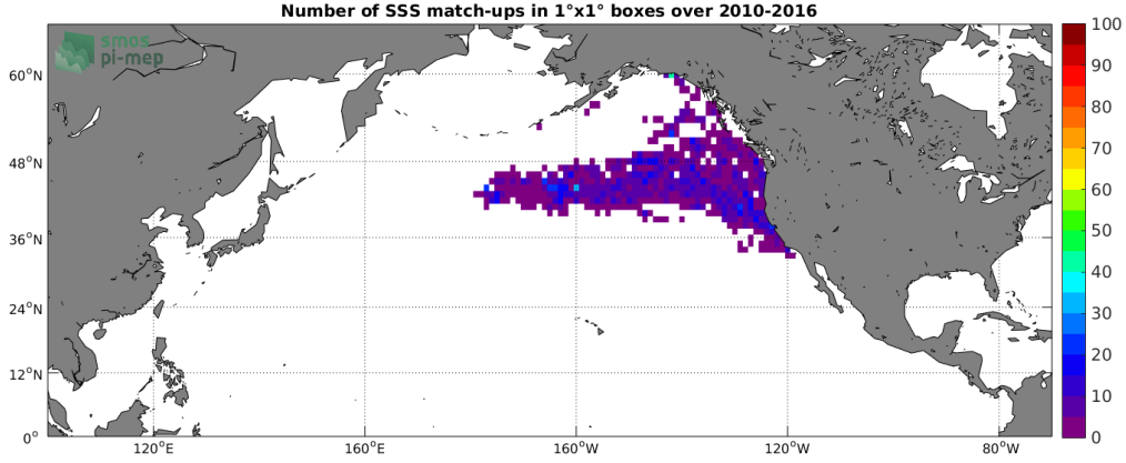
Figure 4: Number of SSS match-ups between Sea mammals SSS and the SMOS SSS L2 v700 (ESA) SSS product for the North Pacific Ocean Pi-MEP region over 1^\circ \times 1^\circ boxes and for the full satellite product period.
