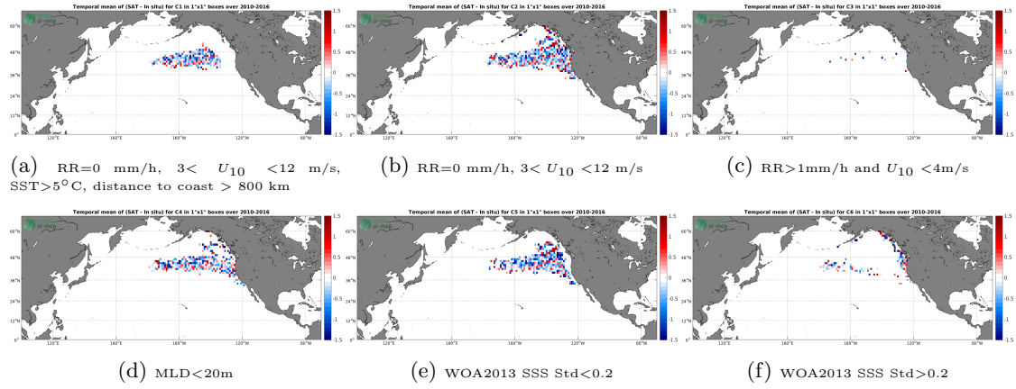
Figure 12: Temporal mean gridded over spatial boxes of size 1^\circ \times 1^\circ of \Delta SSS (SMOS SSS L2 v700 (ESA) - Sea mammals) for 6 different subdatasets corresponding to: RR=0 mm/h, 3 < U_{10} < 12 m/s, SST > 5^\circ C , distance to coast > 800 km (a), RR=0 mm/h, 3 < U_{10} < 12 m/s (b), RR > 1 mm/h and U_{10} < 4 m/s (c), MLD < 20 m (d), WOA2013 SSS Std < 0.2 (e), WOA2013 SSS Std > 0.2 (f).
