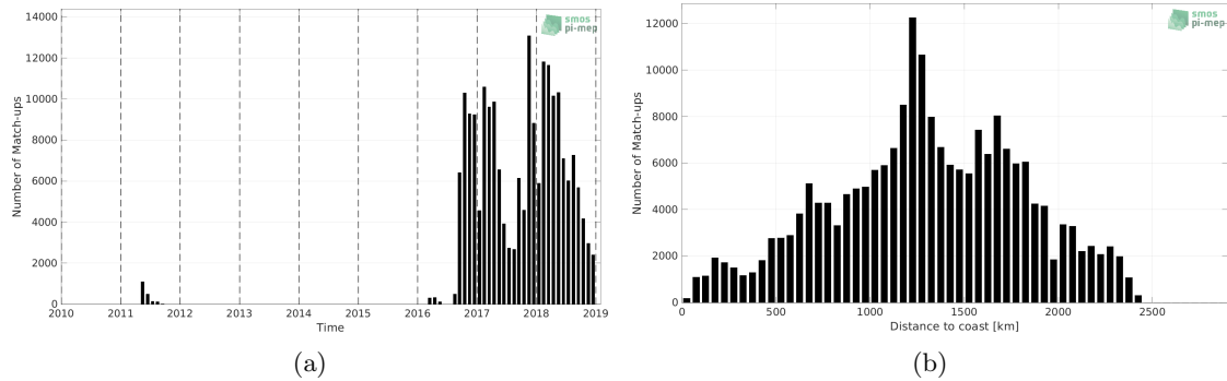
Figure 1: Number of match-ups between Surface drifters and SMOS SSS L2 v700 (ESA) SSS as a function of time (a) and as function of the distance to coast (b) over the North Pacific Ocean Pi-MEP region and for the full satellite product period.
