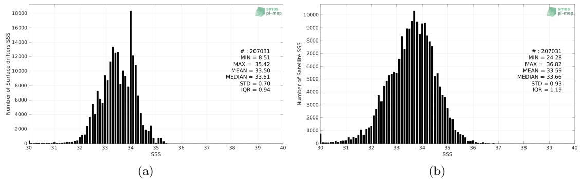
Figure 2: Histograms of SSS from Surface drifters (a) and SMOS SSS L2 v700 (ESA) (b) considering all match-up pairs per bins of 0.1 over the North Pacific Ocean Pi-MEP region and for the full satellite product period.
