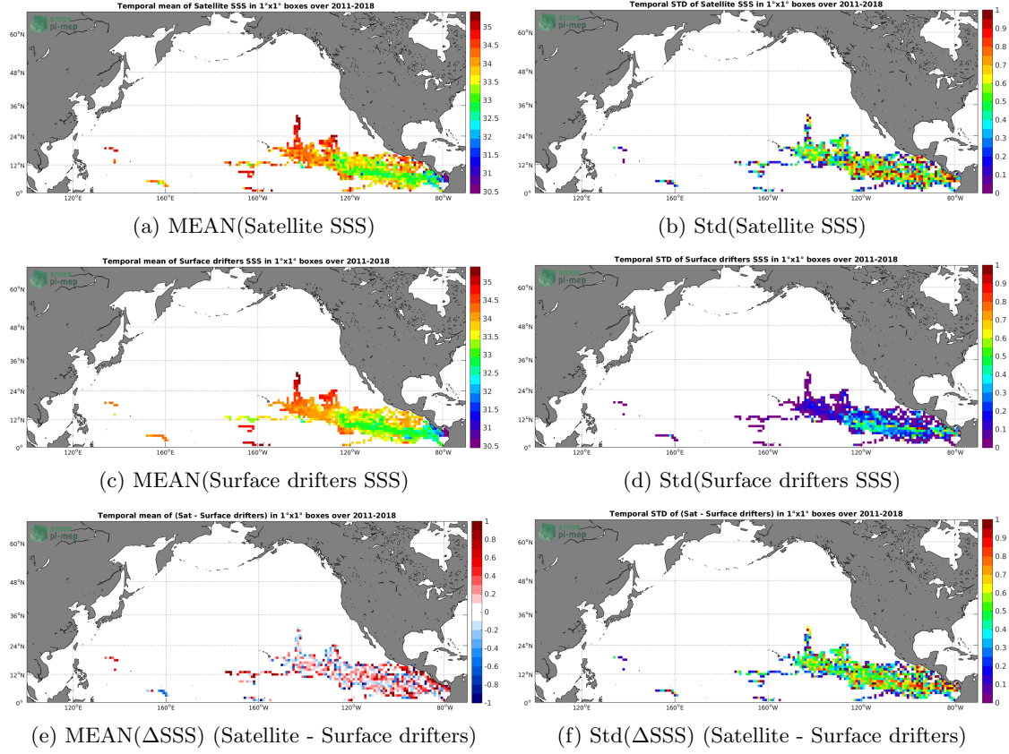
Figure 5: Temporal mean (left) and Std (right) of SSS from SMOS SSS L2 v700 (ESA) (top), Surface drifters (middle), and of \Delta SSS (Satellite - Surface drifters). Only match-up pairs are used to generate these maps.
