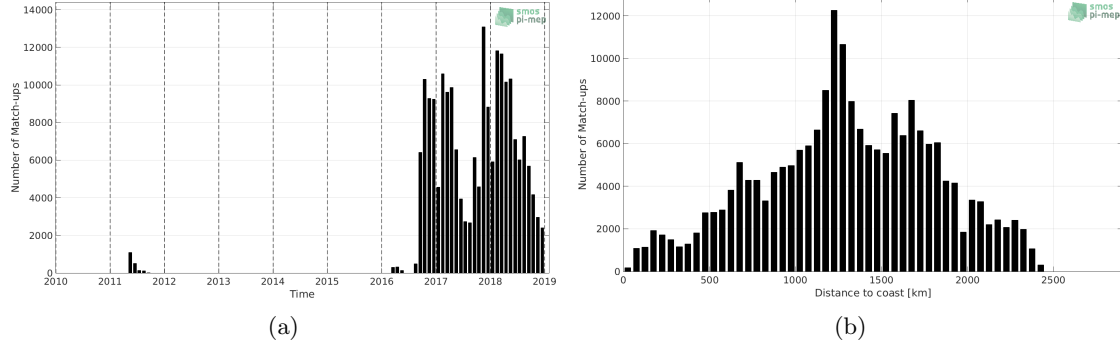
Figure 1: Number of match-ups between Surface drifters and SMOS SSS L2 v700 (ESA) SSS as a function of time (a) and as function of the distance to coast (b) over the North Pacific Ocean Pi-MEP region and for the full satellite product period.
