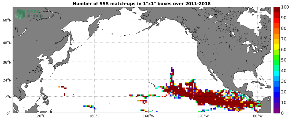
Figure 3: Number of SSS match-ups between Surface drifters SSS and the SMOS SSS L2 v700 (ESA) SSS product for the North Pacific Ocean Pi-MEP region over 1^\circ \times 1^\circ boxes and for the full satellite product period.
