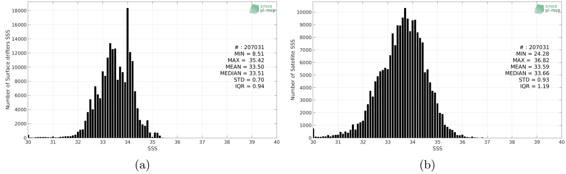
Figure 2: Histograms of SSS from Surface drifters (a) and SMOS SSS L2 v700 (ESA) (b) considering all match-up pairs per bins of 0.1 over the North Pacific Ocean Pi-MEP region and for the full satellite product period.
