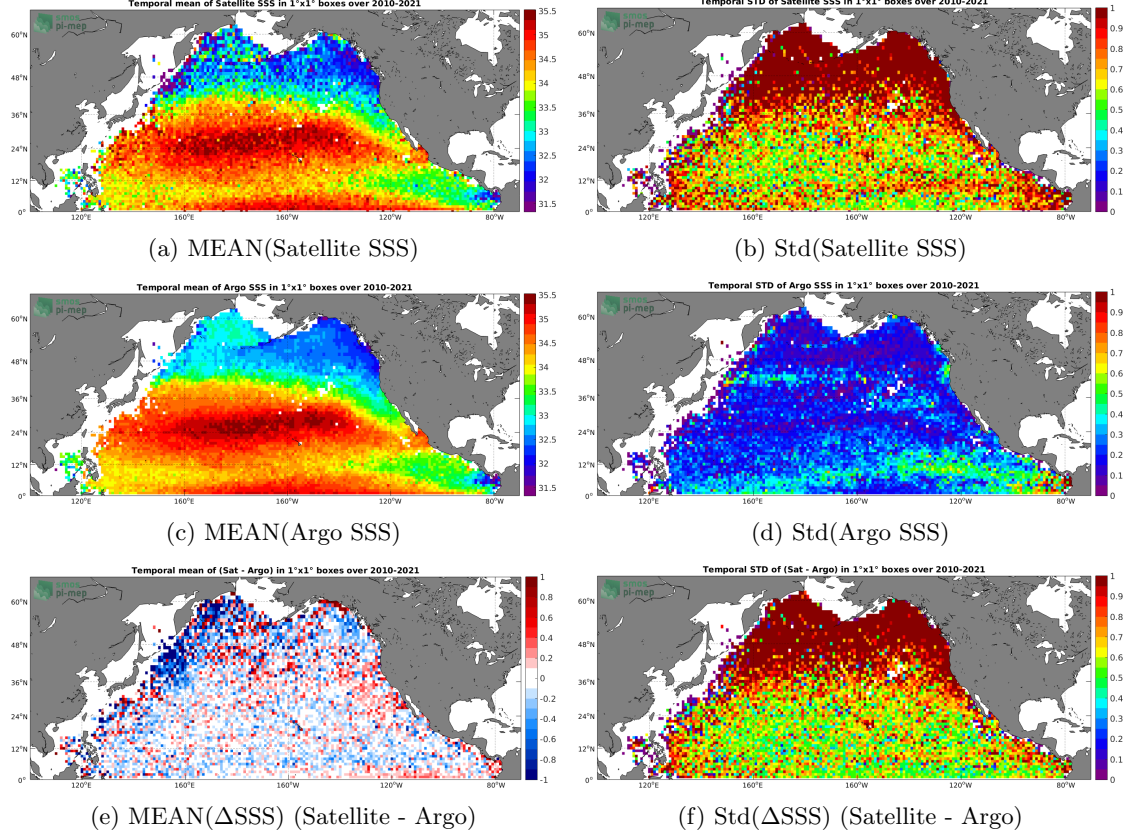
Figure 6: Temporal mean (left) and Std (right) of SSS from SMOS SSS L2 v700 (ESA) (top), Argo (middle), and of \Delta\text{SSS} (Satellite - Argo). Only match-up pairs are used to generate these maps.
