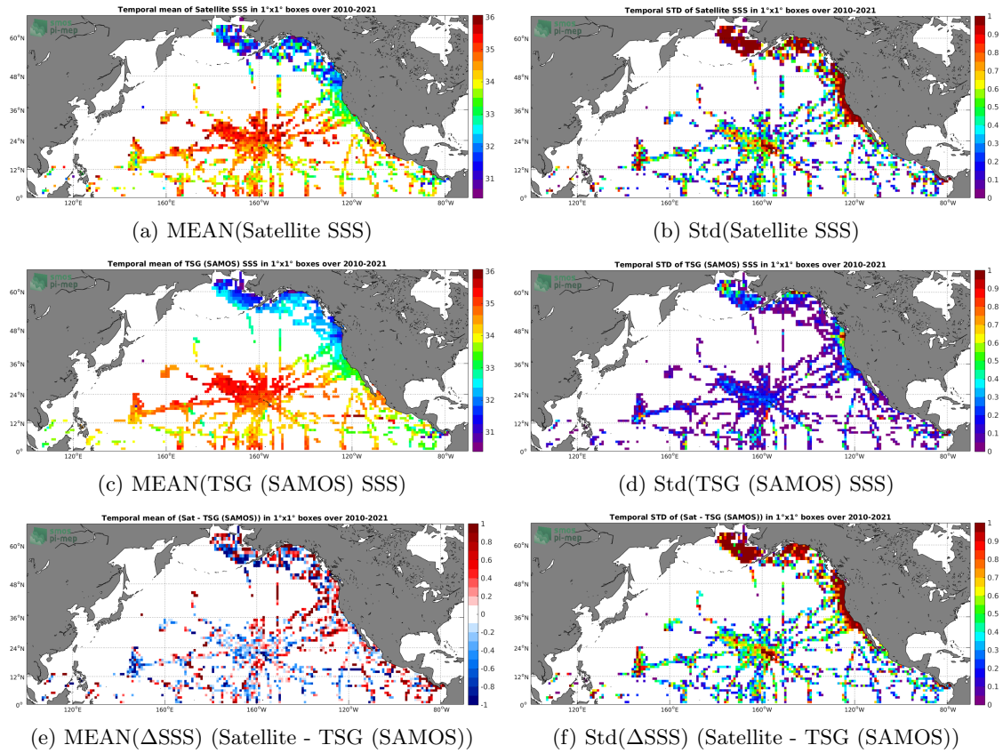
Figure 6: Temporal mean (left) and Std (right) of SSS from SMOS SSS L2 v662 (ESA) (top), TSG (SAMOS) (middle), and of \Delta SSS (Satellite - TSG (SAMOS)). Only match-up pairs are used to generate these maps.
