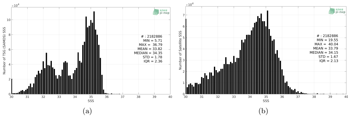
Figure 2: Histograms of SSS from TSG (SAMOS) (a) and SMOS SSS L2 v662 (ESA) (b) considering all match-up pairs per bins of 0.1 over the North Pacific Ocean Pi-MEP region and for the full satellite product period.
