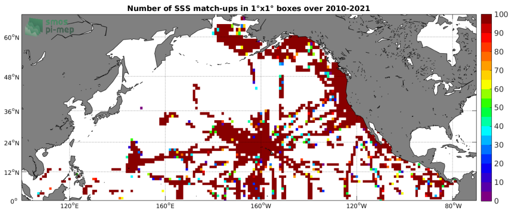
Figure 4: Number of SSS match-ups between TSG (SAMOS) SSS and the SMOS SSS L2 v662 (ESA) SSS product for the North Pacific Ocean Pi-MEP region over 1^\circ \times 1^\circ boxes and for the full satellite product period.
