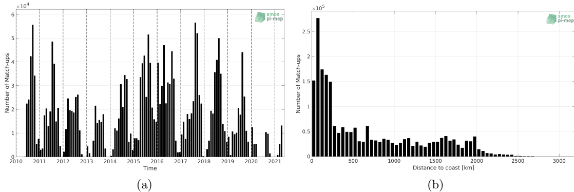
Figure 1: Number of match-ups between TSG (SAMOS) and SMOS SSS L2 v662 (ESA) SSS as a function of time (a) and as function of the distance to coast (b) over the North Pacific Ocean Pi-MEP region and for the full satellite product period.
