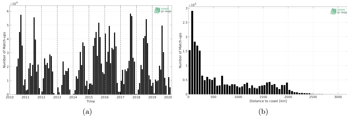
Figure 1: Number of match-ups between TSG-SAMOS and SMOS L2 v662 (ESA) SSS as a function of time (a) and as function of the distance to coast (b) over the North Pacific Ocean Pi-MEP region and for the full satellite product period.
