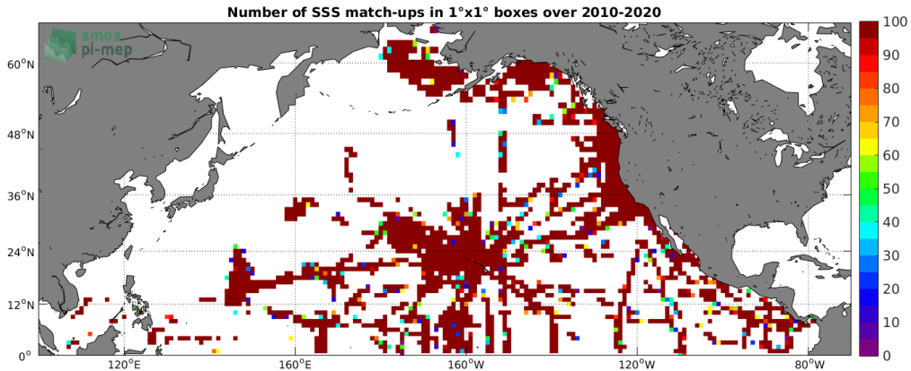
Figure 4: Number of SSS match-ups between TSG-SAMOS SSS and the SMOS L2 v662 (ESA) SSS product for the North Pacific Ocean Pi-MEP region over 1^\circ \times 1^\circ boxes and for the full satellite product period.
