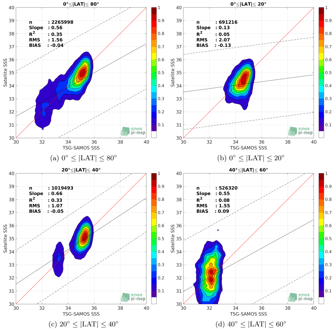
Figure 9: Contour maps of the concentration of SMOS L2 v662 (ESA) SSS ( y -axis) versus TSG-SAMOS SSS ( x -axis) at match-up pairs for different latitude bands. For each plot, the red line shows x=y . The black thin and dashed lines indicate a linear fit through the data cloud and the \pm 95\% confidence levels, respectively. The number match-up pairs n , the slope and R^2 coefficient of the linear fit, the root mean square (RMS) and the mean bias between satellite and in situ data are indicated for each latitude band in each plots.
