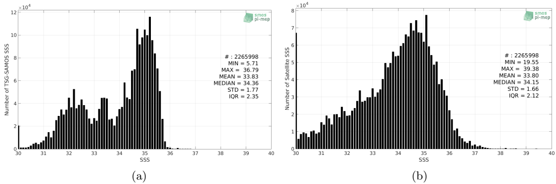
Figure 2: Histograms of SSS from TSG-SAMOS (a) and SMOS L2 v662 (ESA) (b) considering all match-up pairs per bins of 0.1 over the North Pacific Ocean Pi-MEP region and for the full satellite product period.
