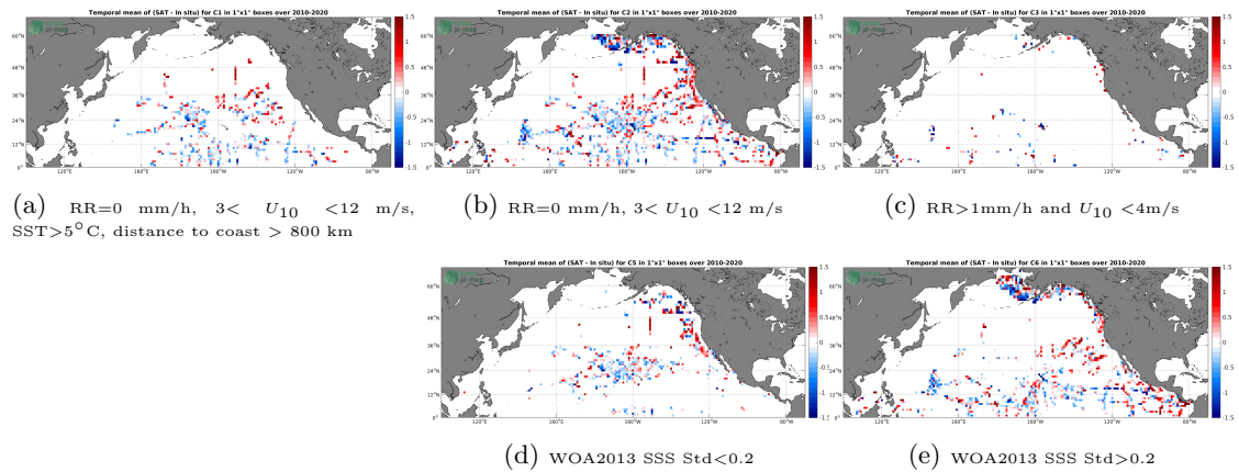
Figure 12: Temporal mean gridded over spatial boxes of size 1^\circ \times 1^\circ of \Delta SSS (SMOS L2 v662 (ESA) - TSG-SAMOS) for 5 different subdatasets corresponding to:RR=0 mm/h, 3 < U_{10} < 12 m/s, SST >5^\circ\text{C} , distance to coast > 800 km (a), RR=0 mm/h, 3 < U_{10} < 12 m/s (b), RR >1 mm/h and U_{10} < 4 m/s (c), WOA2013 SSS Std <0.2 (d), WOA2013 SSS Std >0.2 (e).
