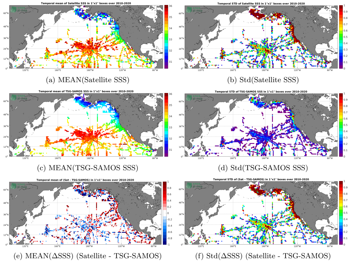
Figure 6: Temporal mean (left) and Std (right) of SSS from SMOS L2 v662 (ESA) (top), TSG-SAMOS (middle), and of \Delta SSS (Satellite - TSG-SAMOS). Only match-up pairs are used to generate these maps.
