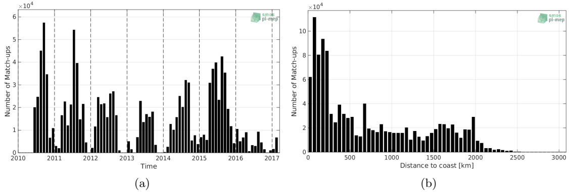
Figure 1: Number of match-ups between TSG-SAMOS and SMOS-L2-DPGS-v662 SSS as a function of time (a) and as function of the distance to coast (b) over the North Pacific Ocean Pi-MEP region and for the full satellite product period.
