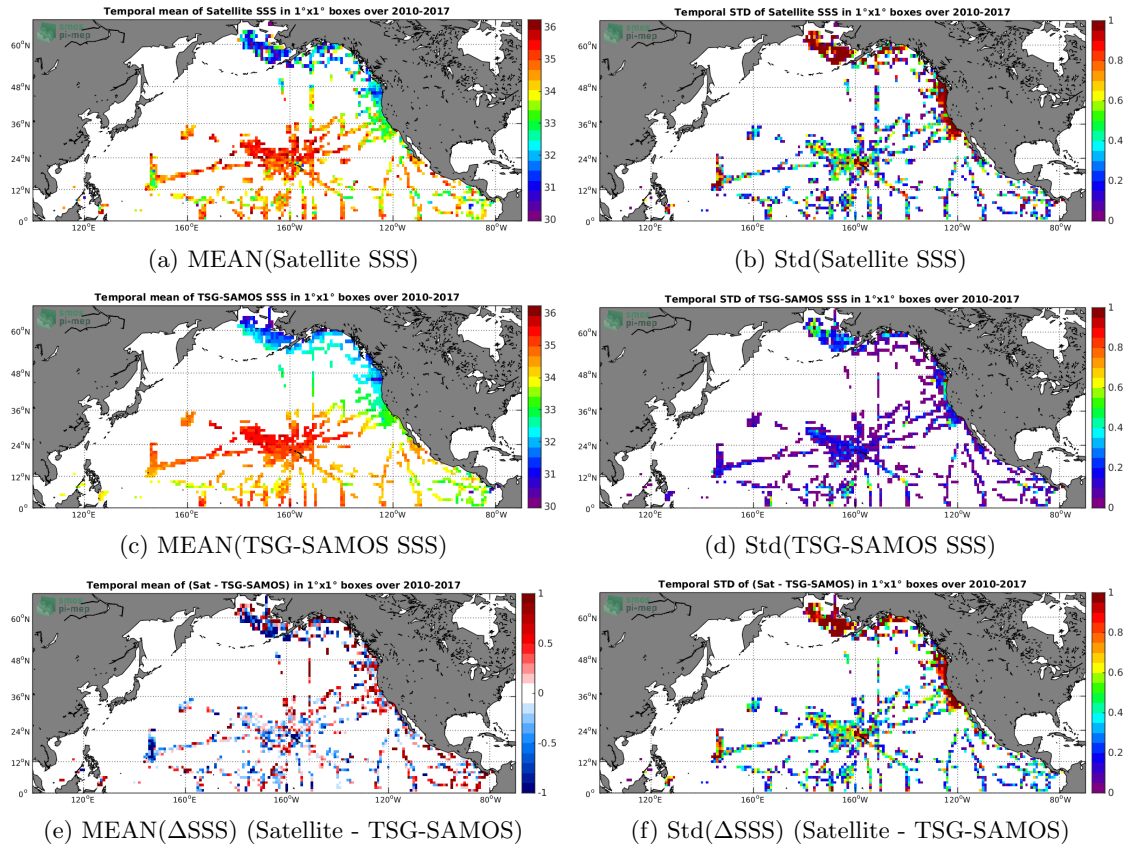
Figure 6: Temporal mean (left) and Std (right) of SSS from SMOS-L2-DPGS-v662 (top), TSG-SAMOS (middle), and of \Delta SSS (Satellite - TSG-SAMOS). Only match-up pairs are used to generate these maps.
