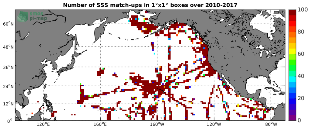
Figure 4: Number of SSS match-ups between TSG-SAMOS SSS and the SMOS-L2-DPGS-v662 SSS product for the North Pacific Ocean Pi-MEP region over 1^\circ \times 1^\circ boxes and for the full satellite product period.
