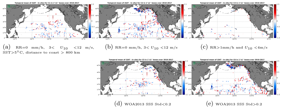
Figure 12: Temporal mean gridded over spatial boxes of size 1^\circ \times 1^\circ of \Delta SSS (SMOS-L2-DPGS-v662 - TSG-SAMOS) for 5 different subdatasets corresponding to:RR=0 mm/h, 3 < U_{10} < 12 m/s, SST >5^\circ\text{C} , distance to coast > 800 km (a), RR=0 mm/h, 3 < U_{10} < 12 m/s (b), RR >1 mm/h and U_{10} < 4 m/s (c), WOA2013 SSS Std <0.2 (d), WOA2013 SSS Std >0.2 (e).
