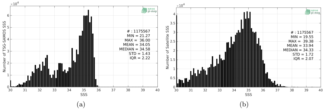
Figure 2: Histograms of SSS from TSG-SAMOS (a) and SMOS-L2-DPGS-v662 (b) considering all match-up pairs per bins of 0.1 over the North Pacific Ocean Pi-MEP region and for the full satellite product period.
