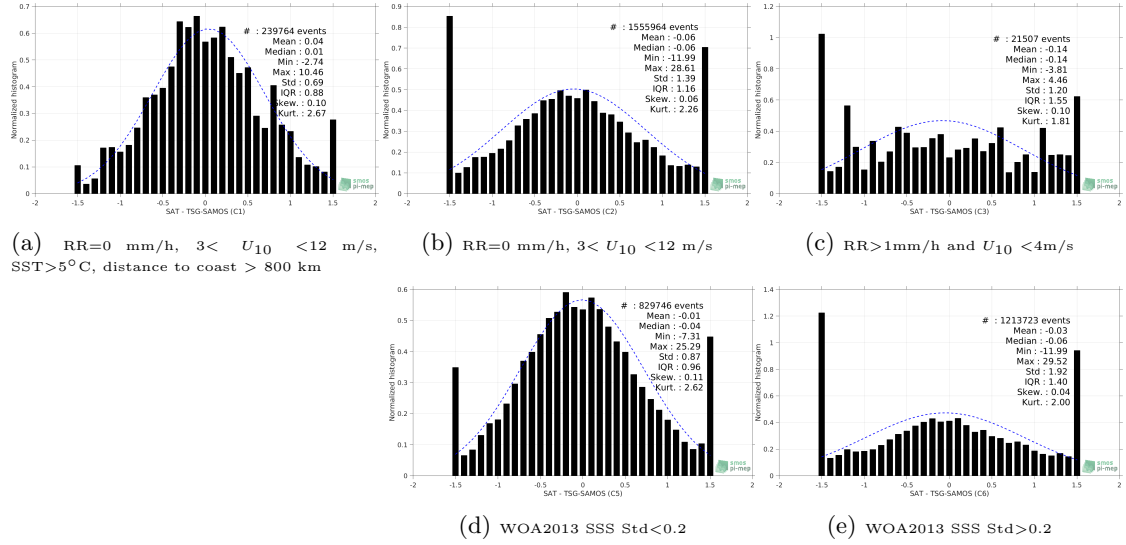
Figure 13: Normalized histogram of \Delta SSS (SMOS-L2-DPGS-v662 - TSG-SAMOS) for 5 different subdatasets corresponding to: RR=0 mm/h, 3 < U_{10} < 12 m/s, SST > 5°C, distance to coast > 800 km (a), RR=0 mm/h, 3 < U_{10} < 12 m/s (b), RR > 1mm/h and U_{10} < 4 m/s (c), WOA2013 SSS Std < 0.2 (d), WOA2013 SSS Std > 0.2 (e).
