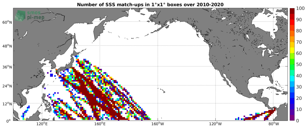
Figure 4: Number of SSS match-ups between TSG (LEGOS-DM) SSS and the SMOS SSS L2 v662 (ESA) SSS product for the North Pacific Ocean Pi-MEP region over 1^\circ \times 1^\circ boxes and for the full satellite product period.
