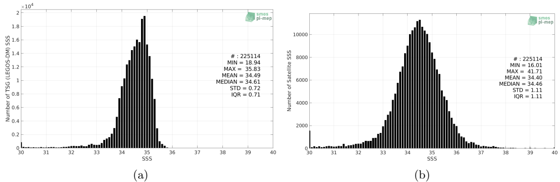
Figure 2: Histograms of SSS from TSG (LEGOS-DM) (a) and SMOS SSS L2 v662 (ESA) (b) considering all match-up pairs per bins of 0.1 over the North Pacific Ocean Pi-MEP region and for the full satellite product period.
