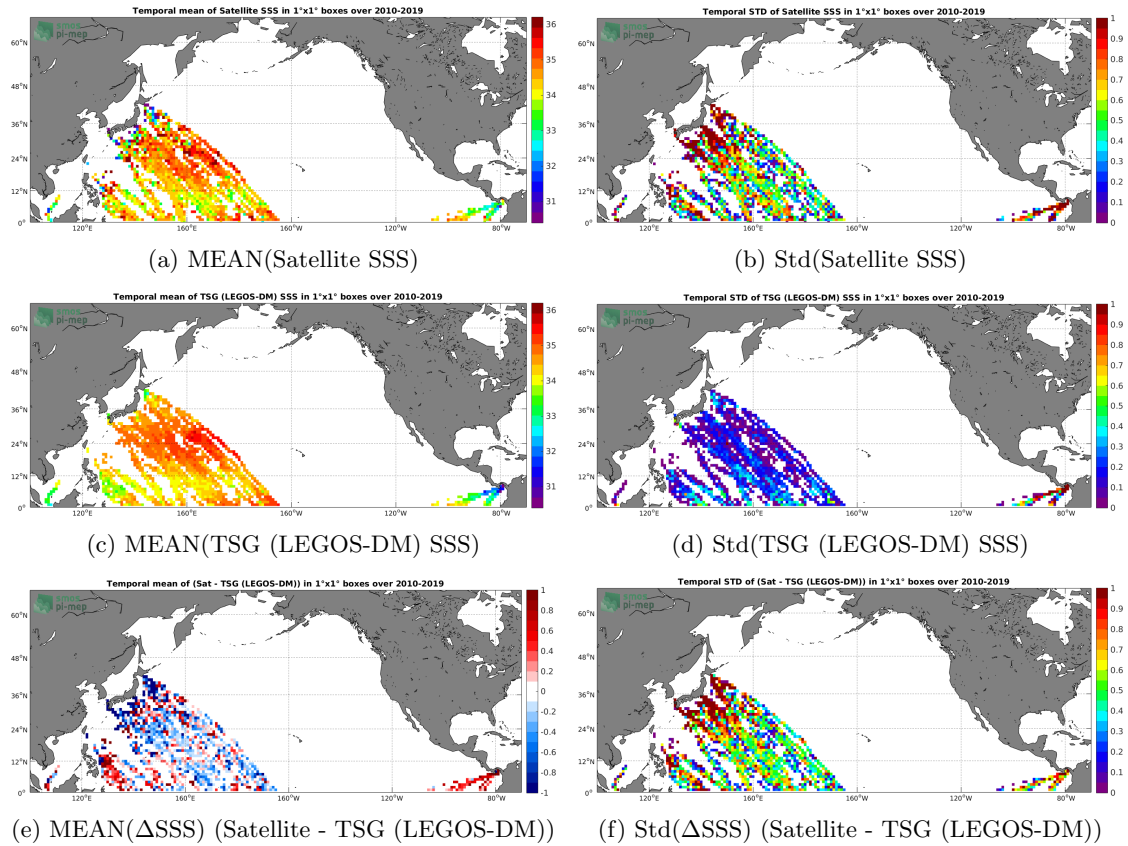
Figure 6: Temporal mean (left) and Std (right) of SSS from SMOS SSS L2 v662 (ESA) (top), TSG (LEGOS-DM) (middle), and of \Delta SSS (Satellite - TSG (LEGOS-DM)). Only match-up pairs are used to generate these maps.
