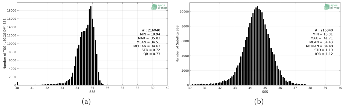
Figure 2: Histograms of SSS from TSG (LEGOS-DM) (a) and SMOS SSS L2 v662 (ESA) (b) considering all match-up pairs per bins of 0.1 over the North Pacific Ocean Pi-MEP region and for the full satellite product period.
