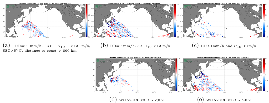
Figure 12: Temporal mean gridded over spatial boxes of size 1°x1° of \Delta SSS (SMOS SSS L2 v662 (ESA) - TSG (LEGOS-DM)) for 5 different subdatasets corresponding to:RR=0 mm/h, 3 < U_{10} < 12 m/s, SST>5°C, distance to coast > 800 km (a), RR=0 mm/h, 3 < U_{10} < 12 m/s (b), RR>1mm/h and U_{10} < 4 m/s (c), WOA2013 SSS Std<0.2 (d), WOA2013 SSS Std>0.2 (e).
