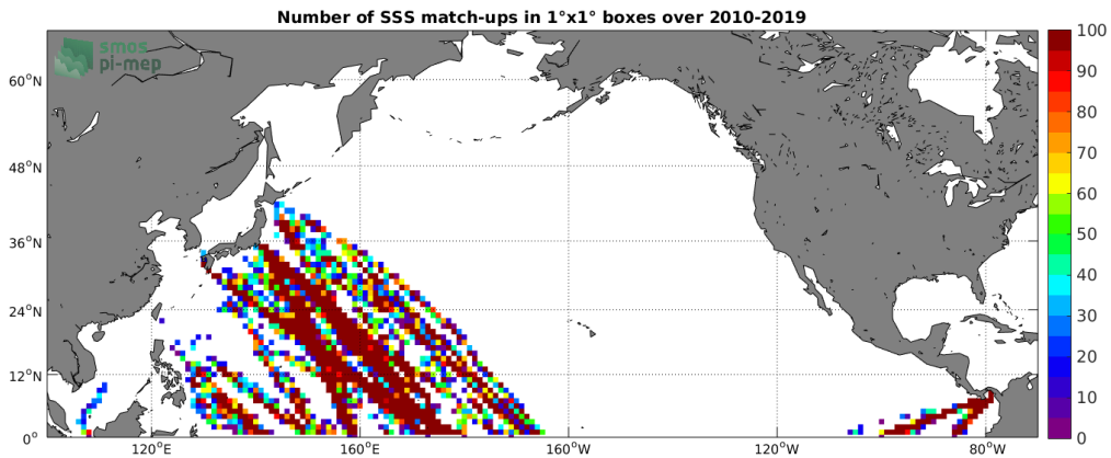
Figure 4: Number of SSS match-ups between TSG (LEGOS-DM) SSS and the SMOS SSS L2 v662 (ESA) SSS product for the North Pacific Ocean Pi-MEP region over 1°x1° boxes and for the full satellite product period.
