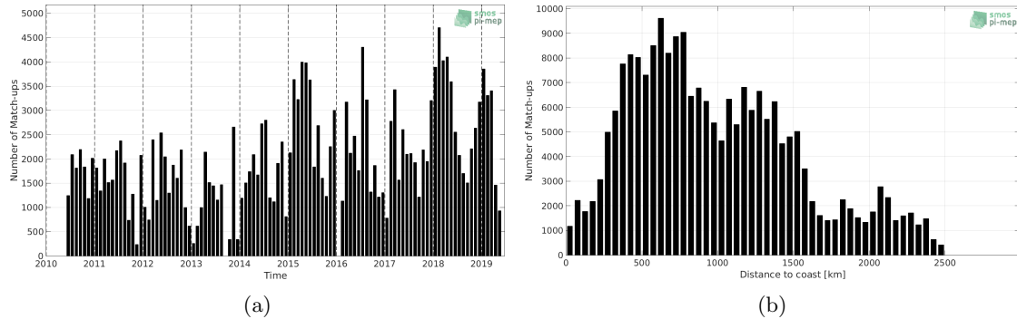
Figure 1: Number of match-ups between TSG (LEGOS-DM) and SMOS SSS L2 v662 (ESA) SSS as a function of time (a) and as function of the distance to coast (b) over the North Pacific Ocean Pi-MEP region and for the full satellite product period.
