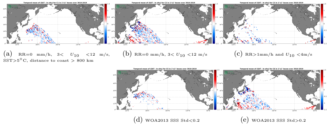
Figure 12: Temporal mean gridded over spatial boxes of size 1^\circ \times 1^\circ of \Delta SSS (SMOS L2 v662 (ESA) - TSG-LEGOS-DM) for 5 different subdatasets corresponding to:RR=0 mm/h, 3 < U_{10} < 12 m/s, SST >5^\circ\text{C} , distance to coast > 800 km (a), RR=0 mm/h, 3 < U_{10} < 12 m/s (b), RR >1 mm/h and U_{10} < 4 m/s (c), WOA2013 SSS Std <0.2 (d), WOA2013 SSS Std >0.2 (e).
