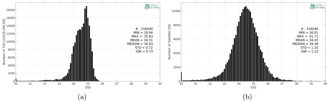
Figure 2: Histograms of SSS from TSG-LEGOS-DM (a) and SMOS L2 v662 (ESA) (b) considering all match-up pairs per bins of 0.1 over the North Pacific Ocean Pi-MEP region and for the full satellite product period.
