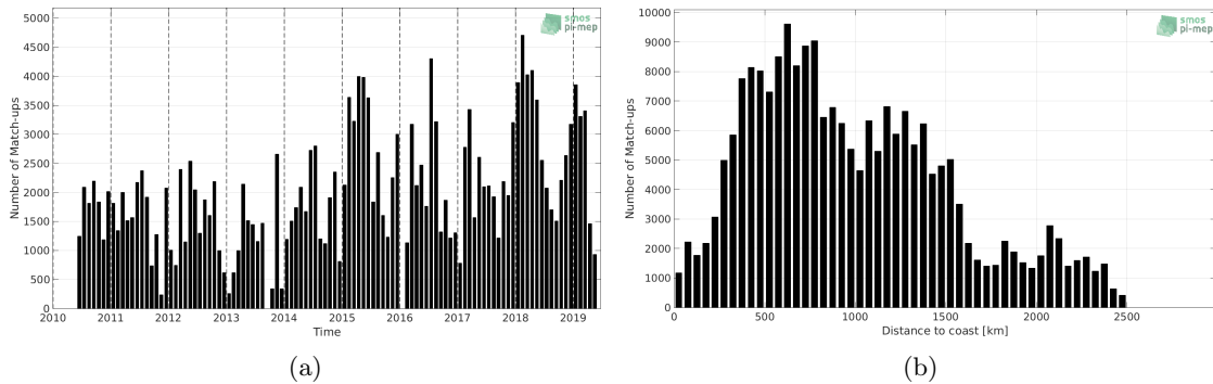
Figure 1: Number of match-ups between TSG-LEGOS-DM and SMOS L2 v662 (ESA) SSS as a function of time (a) and as function of the distance to coast (b) over the North Pacific Ocean Pi-MEP region and for the full satellite product period.
