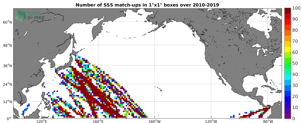
Figure 4: Number of SSS match-ups between TSG-LEGOS-DM SSS and the SMOS L2 v662 (ESA) SSS product for the North Pacific Ocean Pi-MEP region over 1^\circ \times 1^\circ boxes and for the full satellite product period.
