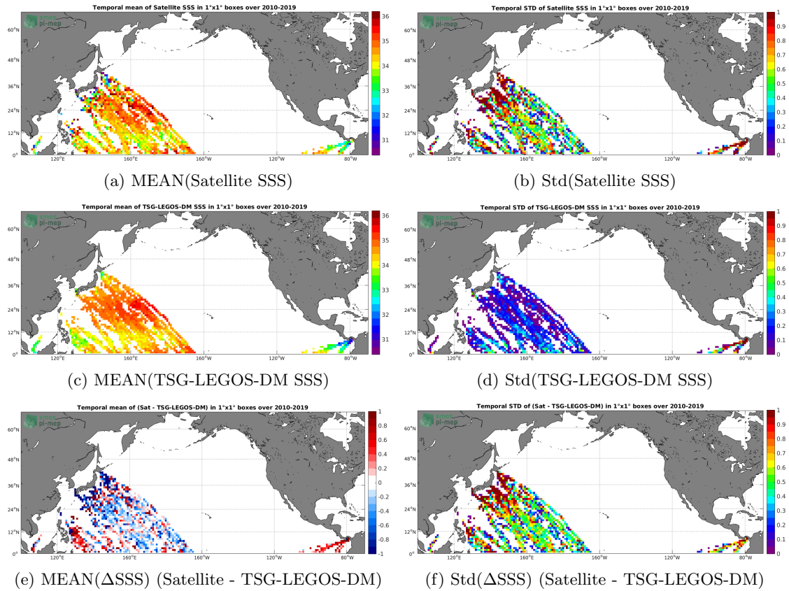
Figure 6: Temporal mean (left) and Std (right) of SSS from SMOS L2 v662 (ESA) (top), TSG-LEGOS-DM (middle), and of \Delta SSS (Satellite - TSG-LEGOS-DM). Only match-up pairs are used to generate these maps.
