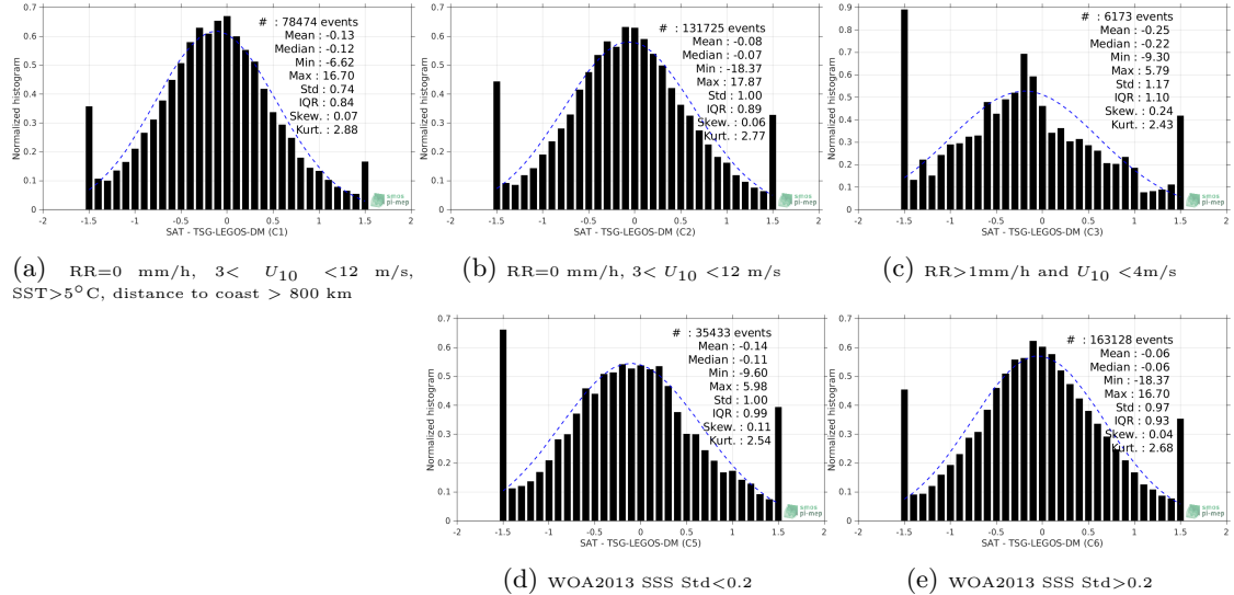
Figure 13: Normalized histogram of \Delta\text{SSS} (SMOS-L2-DPGS-v662 - TSG-LEGOS-DM) for 5 different subdatasets corresponding to: RR=0 mm/h, 3 < U_{10} < 12 m/s, SST>5°C, distance to coast > 800 km (a), RR=0 mm/h, 3 < U_{10} < 12 m/s (b), RR>1mm/h and U_{10} < 4 m/s (c), WOA2013 SSS Std<0.2 (d), WOA2013 SSS Std>0.2 (e).
