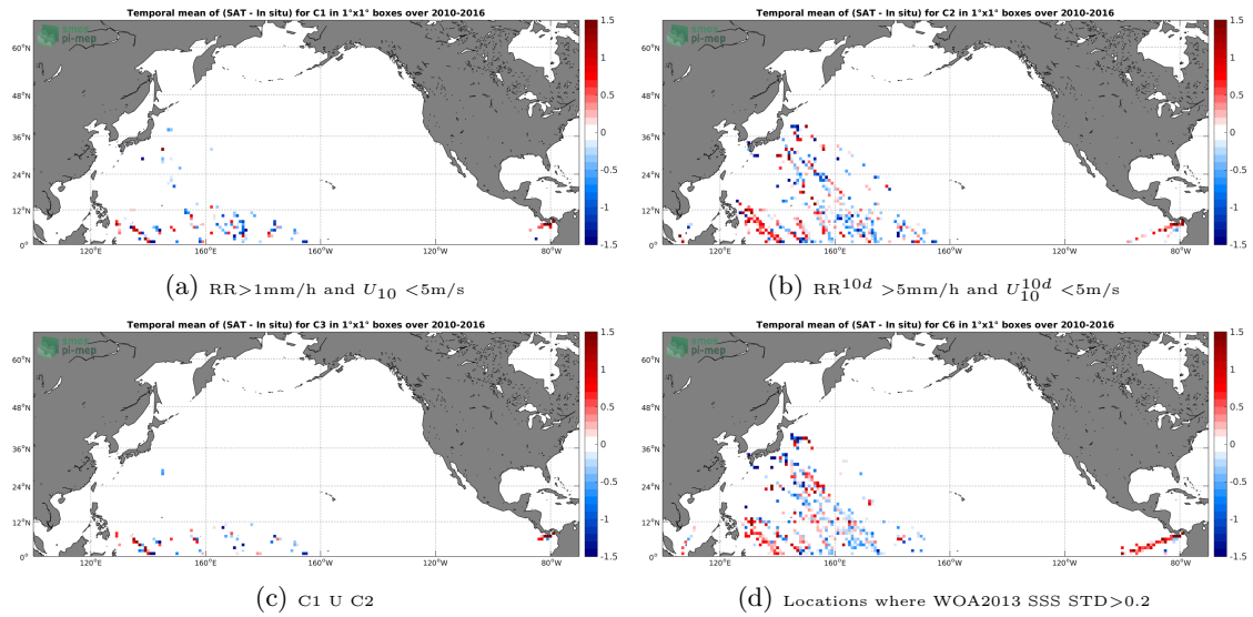
Figure 12: Temporal mean gridded over spatial boxes of size 1^\circ \times 1^\circ of \Delta SSS (SMOS-L2-DPGS-v662 - TSG-LEGOS-DM) for 4 different subdatasets corresponding to: RR > 1 mm/h and U_{10} < 5 m/s (a), RR 10d > 5 mm/h and U_{10}^{10d} < 5 m/s (b), C1 U C2 (c), Locations where WOA2013 SSS STD > 0.2 (d).
