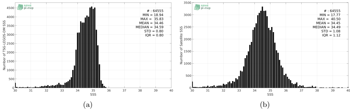
Figure 2: Histograms of SSS from TSG-LEGOS-DM (a) and SMOS-L2-DPGS-v662 (b) considering all match-up pairs per bins of 0.1 over the North Pacific Ocean Pi-MEP region and for the full satellite product period.
