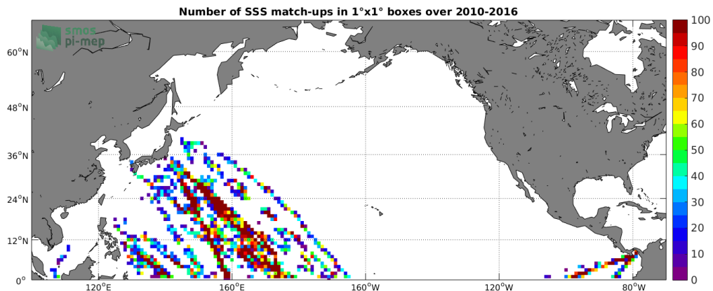
Figure 4: Number of SSS match-ups between TSG-LEGOS-DM SSS and the SMOS-L2-DPGS-v662 SSS product for the North Pacific Ocean Pi-MEP region over 1^\circ \times 1^\circ boxes and for the full satellite product period.
