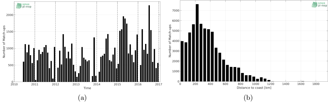
Figure 1: Number of match-ups between TSG-LEGOS-DM and SMOS-L2-DPGS-v662 SSS as a function of time (a) and as function of the distance to coast (b) over the North Pacific Ocean Pi-MEP region and for the full satellite product period.
