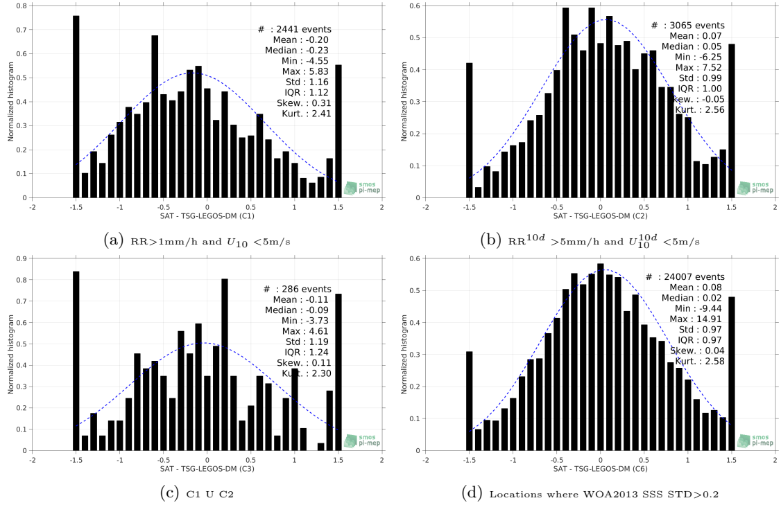
Figure 13: Normalized histogram of \Delta SSS (SMOS-L2-DPGS-v662 - TSG-LEGOS-DM) for 6 different subdatasets corresponding to: RR > 1\text{mm/h} and U_{10} < 5\text{m/s} (a), RR^{10d} > 5\text{mm/h} and U_{10}^{10d} < 5\text{m/s} (b), C1 U C2 (c), Locations where WOA2013 SSS STD > 0.2 (d).
