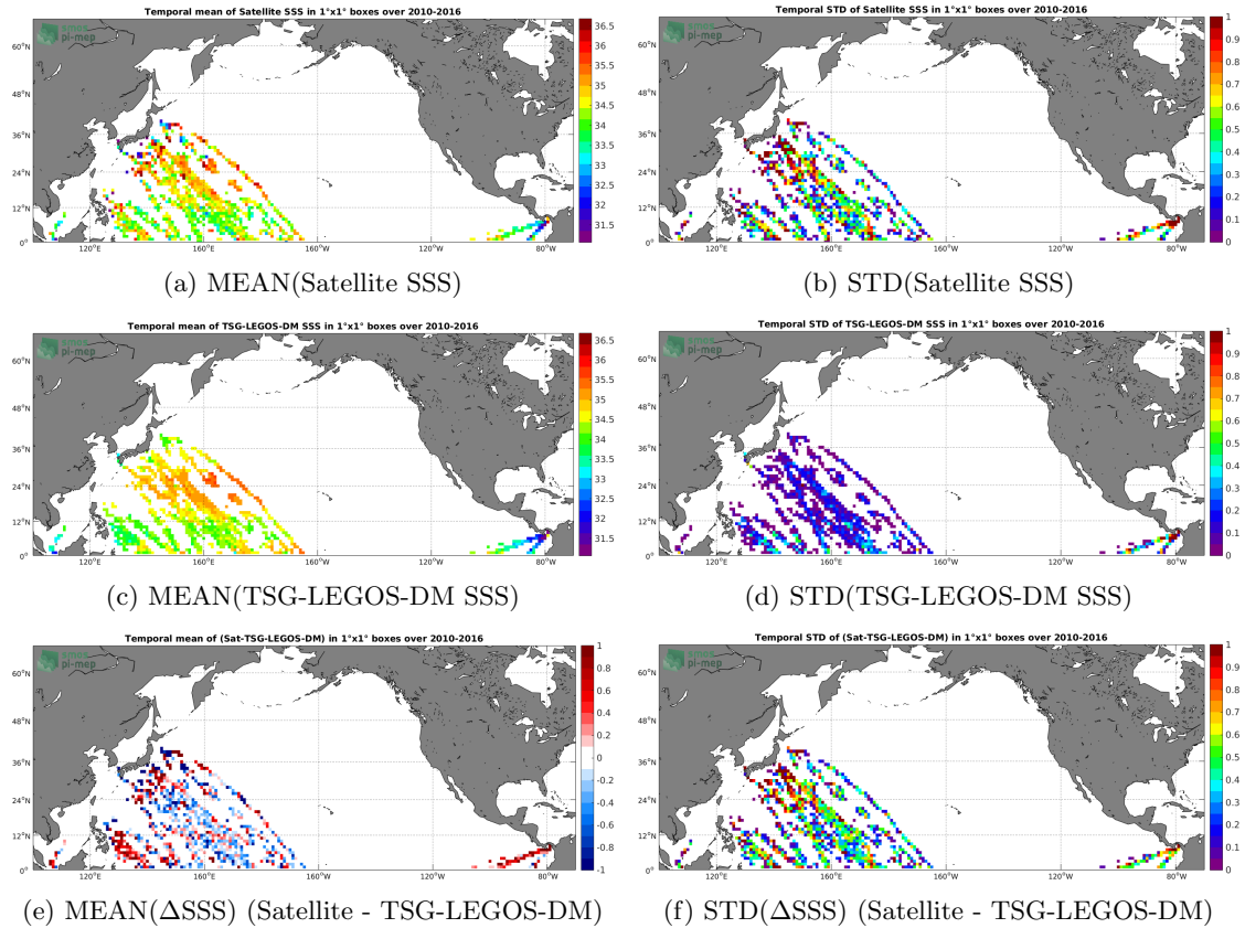
Figure 6: Temporal mean (left) and STD (right) of SSS from SMOS-L2-DPGS-v662 (top), TSG-LEGOS-DM (middle), and of \Delta SSS (Satellite - TSG-LEGOS-DM). Only match-up pairs are used to generate these maps.
