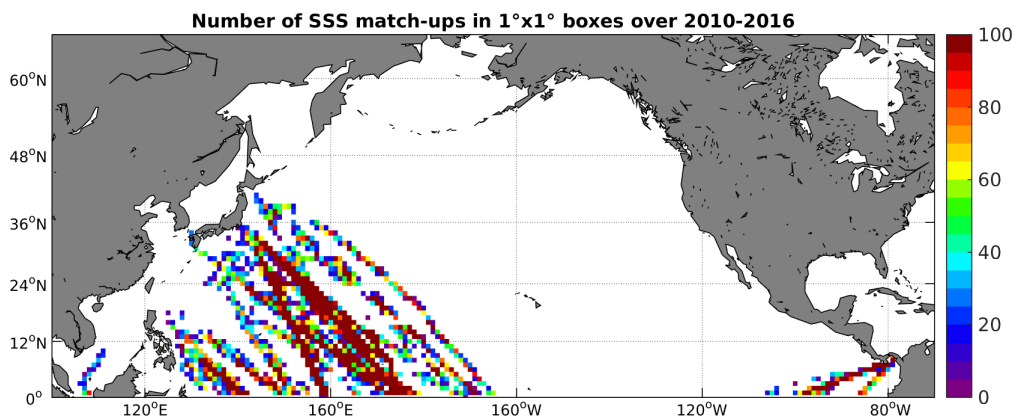
Figure 4: Number of SSS match-ups between TSG-LEGOS-DM SSS and the SMOS-L2-DPGS-v662 SSS product for the North Pacific Ocean Pi-MEP region over 1°x1° boxes and for the full satellite product period.
