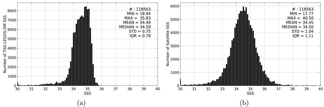
Figure 2: Histograms of SSS from TSG-LEGOS-DM (a) and SMOS-L2-DPGS-v662 (b) considering all match-up pairs per bins of 0.1 over the North Pacific Ocean Pi-MEP region and for the full satellite product period.
