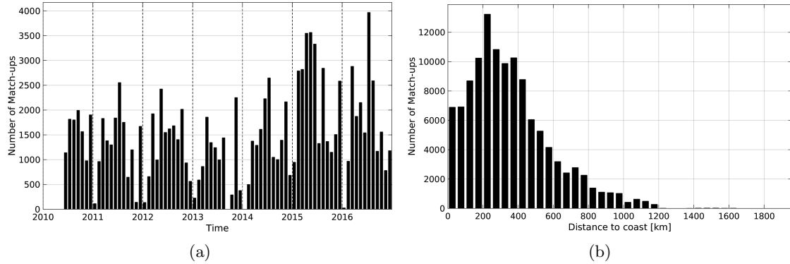
Figure 1: Number of match-ups between TSG-LEGOS-DM and SMOS-L2-DPGS-v662 SSS as a function of time (a) and as function of the distance to coast (b) over the North Pacific Ocean Pi-MEP region and for the full satellite product period.
