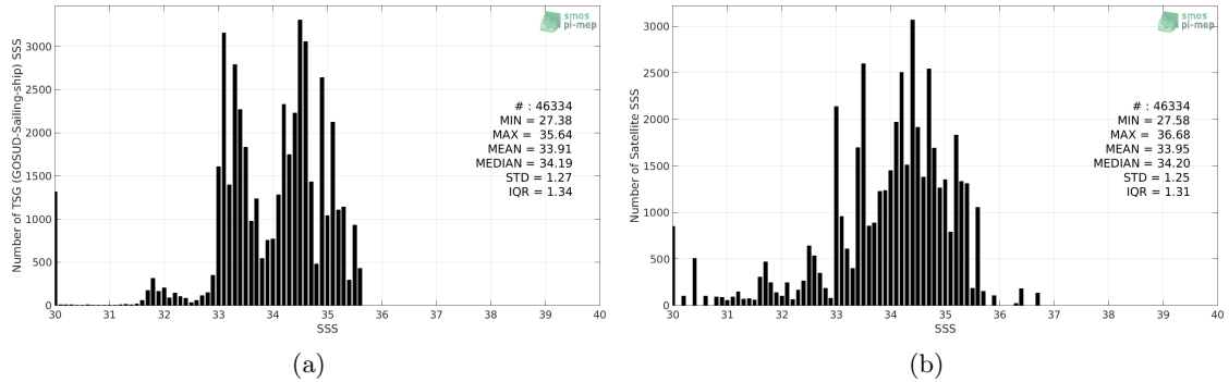
Figure 2: Histograms of SSS from TSG (GOSUD-Sailing-ship) (a) and SMOS SSS L2 v662 (ESA) (b) considering all match-up pairs per bins of 0.1 over the North Pacific Ocean Pi-MEP region and for the full satellite product period.
