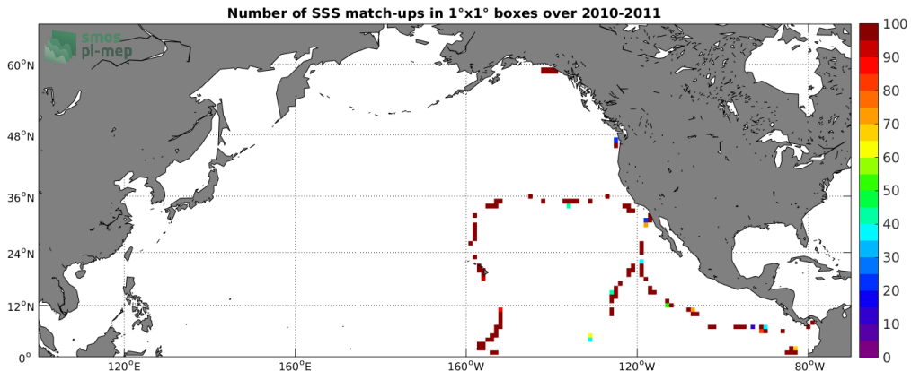
Figure 4: Number of SSS match-ups between TSG (GOSUD-Sailing-ship) SSS and the SMOS SSS L2 v662 (ESA) SSS product for the North Pacific Ocean Pi-MEP region over 1^\circ \times 1^\circ boxes and for the full satellite product period.
