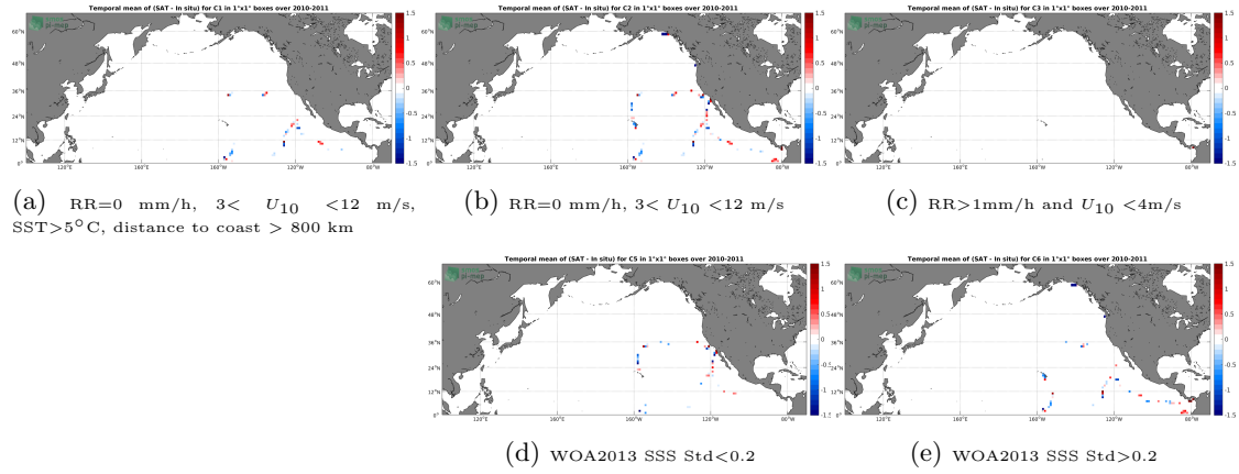
Figure 12: Temporal mean gridded over spatial boxes of size 1^\circ \times 1^\circ of \Delta SSS (SMOS SSS L2 v662 (ESA) - TSG (GOSUD-Sailing-ship)) for 5 different subdatasets corresponding to:RR=0 mm/h, 3 < U_{10} < 12 m/s, SST >5^\circ\text{C} , distance to coast > 800 km (a), RR=0 mm/h, 3 < U_{10} < 12 m/s (b), RR >1 mm/h and U_{10} < 4 m/s (c), WOA2013 SSS Std <0.2 (d), WOA2013 SSS Std >0.2 (e).
