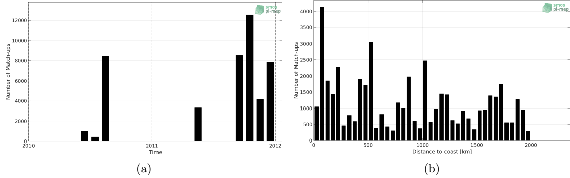
Figure 1: Number of match-ups between TSG (GOSUD-Sailing-ship) and SMOS SSS L2 v662 (ESA) SSS as a function of time (a) and as function of the distance to coast (b) over the North Pacific Ocean Pi-MEP region and for the full satellite product period.
