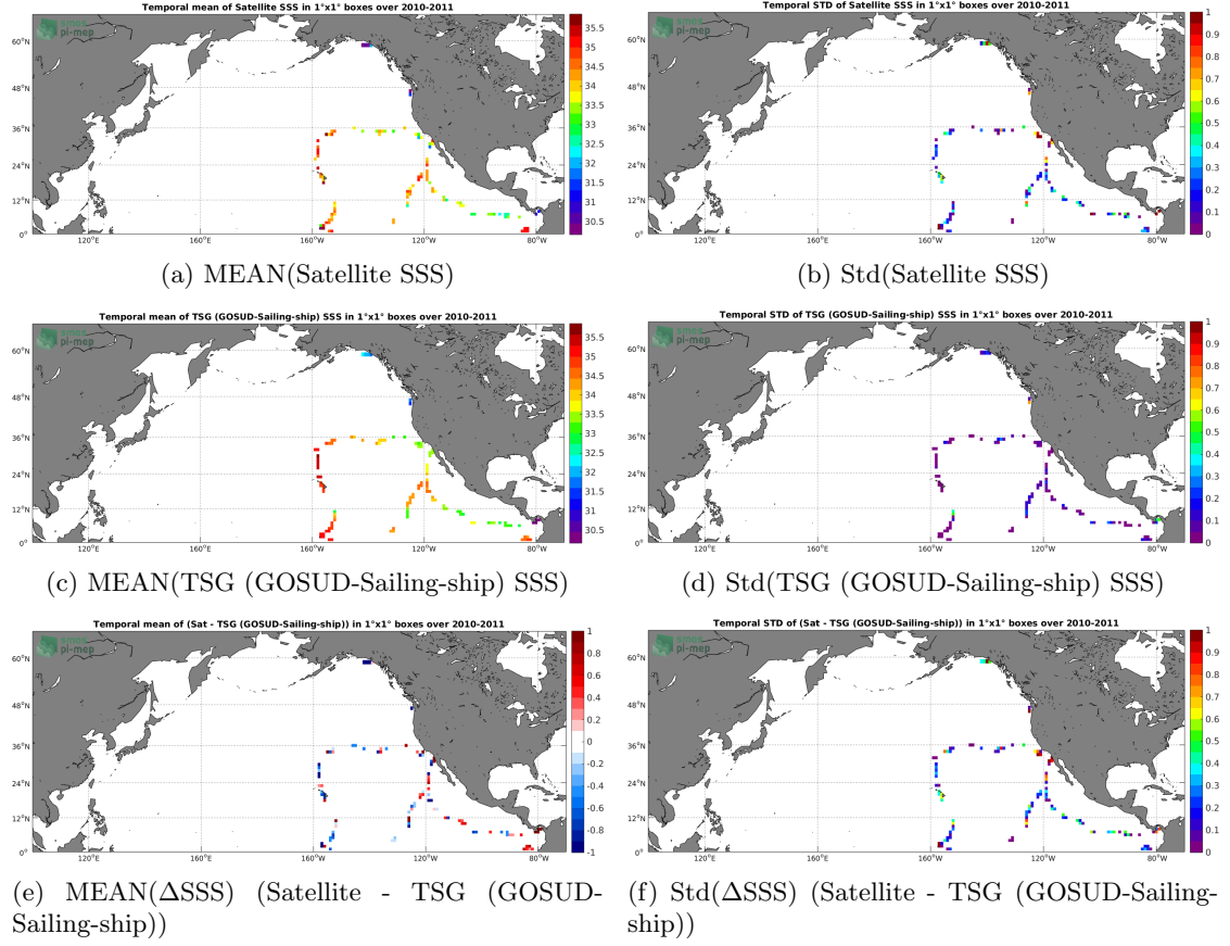
Figure 6: Temporal mean (left) and Std (right) of SSS from SMOS SSS L2 v662 (ESA) (top), TSG (GOSUD-Sailing-ship) (middle), and of \Delta SSS (Satellite - TSG (GOSUD-Sailing-ship)). Only match-up pairs are used to generate these maps.
