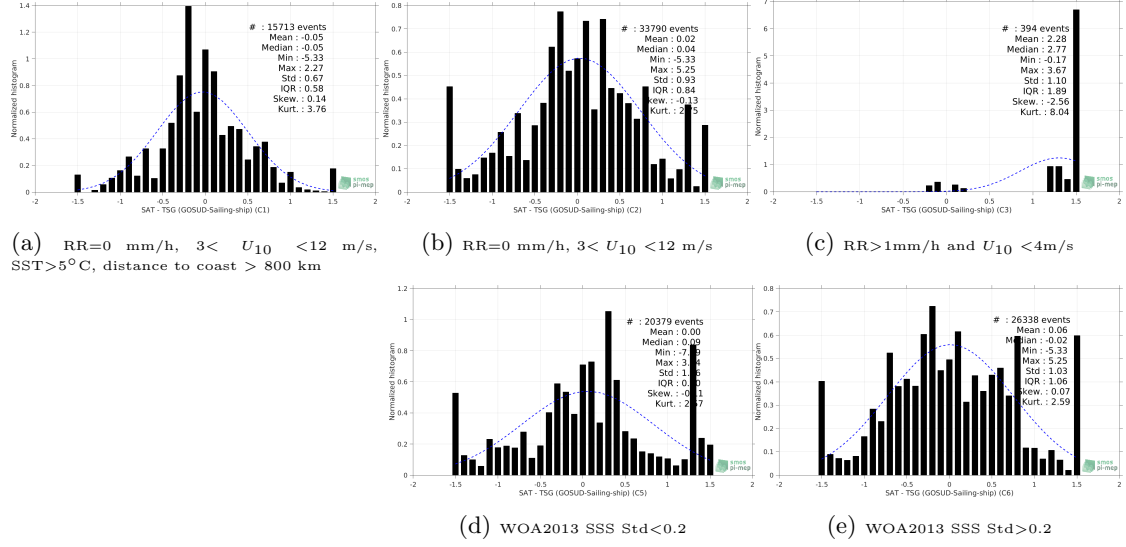
Figure 13: Normalized histogram of \Delta SSS (SMOS SSS L2 v662 (ESA) - TSG (GOSUD-Sailing-ship)) for 5 different subdatasets corresponding to: RR=0 mm/h, 3 < U_{10} < 12 m/s, SST > 5°C, distance to coast > 800 km (a), RR=0 mm/h, 3 < U_{10} < 12 m/s (b), RR > 1mm/h and U_{10} < 4 m/s (c), WOA2013 SSS Std < 0.2 (d), WOA2013 SSS Std > 0.2 (e).
