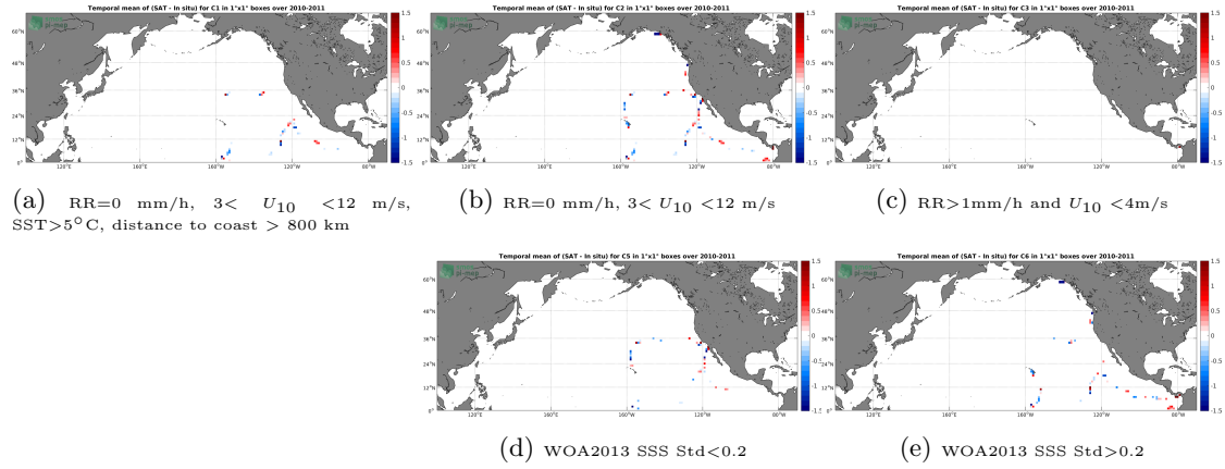
Figure 12: Temporal mean gridded over spatial boxes of size 1^\circ \times 1^\circ of \Delta SSS (SMOS SSS L2 v662 (ESA) - TSG (GOSUD-Sailing-ship)) for 5 different subdatasets corresponding to: RR=0 mm/h, 3 < U_{10} < 12 m/s, SST >5^\circ\text{C} , distance to coast > 800 km (a), RR=0 mm/h, 3 < U_{10} < 12 m/s (b), RR >1 mm/h and U_{10} < 4 m/s (c), WOA2013 SSS Std <0.2 (d), WOA2013 SSS Std >0.2 (e).
