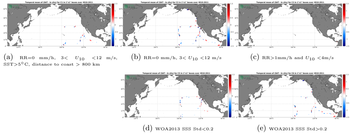
Figure 12: Temporal mean gridded over spatial boxes of size 1^\circ \times 1^\circ of \Delta SSS (SMOS L2 v662 (ESA) - TSG-GOSUD-Sailing-ship) for 5 different subdatasets corresponding to:RR=0 mm/h, 3 < U_{10} < 12 m/s, SST >5^\circ\text{C} , distance to coast > 800 km (a), RR=0 mm/h, 3 < U_{10} < 12 m/s (b), RR >1 mm/h and U_{10} < 4 m/s (c), WOA2013 SSS Std <0.2 (d), WOA2013 SSS Std >0.2 (e).
