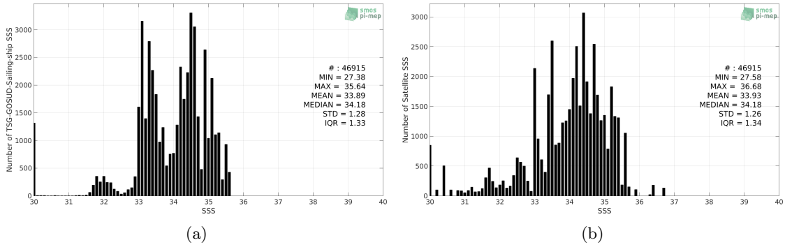
Figure 2: Histograms of SSS from TSG-GOSUD-Sailing-ship (a) and SMOS L2 v662 (ESA) (b) considering all match-up pairs per bins of 0.1 over the North Pacific Ocean Pi-MEP region and for the full satellite product period.
