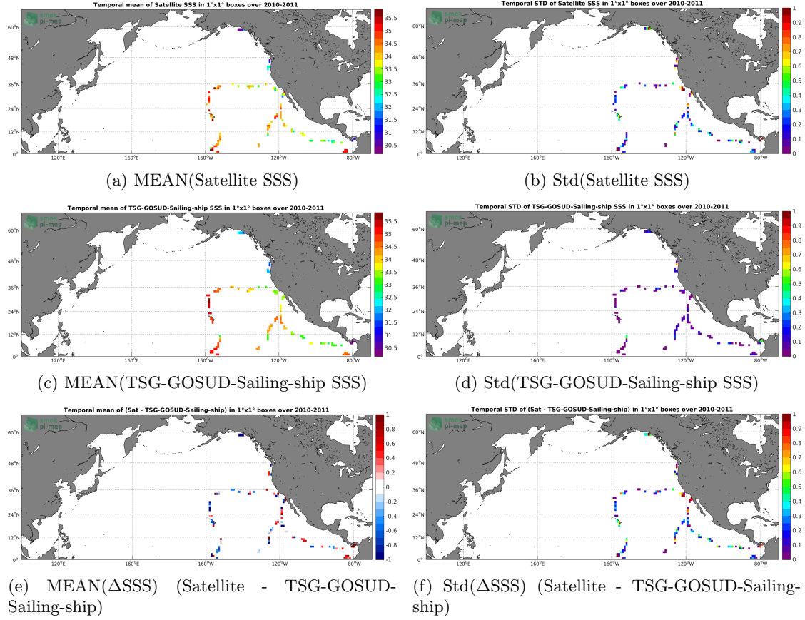
Figure 6: Temporal mean (left) and Std (right) of SSS from SMOS L2 v662 (ESA) (top), TSG-GOSUD-Sailing-ship (middle), and of \Delta SSS (Satellite - TSG-GOSUD-Sailing-ship). Only match-up pairs are used to generate these maps.
