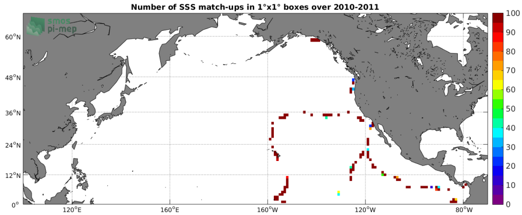
Figure 4: Number of SSS match-ups between TSG-GOSUD-Sailing-ship SSS and the SMOS L2 v662 (ESA) SSS product for the North Pacific Ocean Pi-MEP region over 1°x1° boxes and for the full satellite product period.
