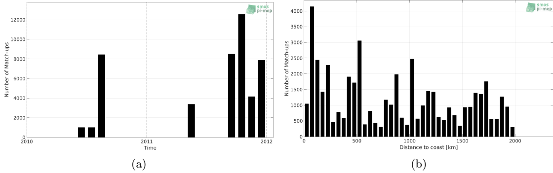
Figure 1: Number of match-ups between TSG-GOSUD-Sailing-ship and SMOS L2 v662 (ESA) SSS as a function of time (a) and as function of the distance to coast (b) over the North Pacific Ocean Pi-MEP region and for the full satellite product period.
