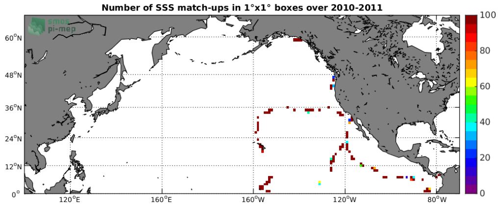
Figure 4: Number of SSS match-ups between TSG-GOSUD-Sailing-ship SSS and the SMOS-L2-DPGS-v662 SSS product for the North Pacific Ocean Pi-MEP region over 1°x1° boxes and for the full satellite product period.
