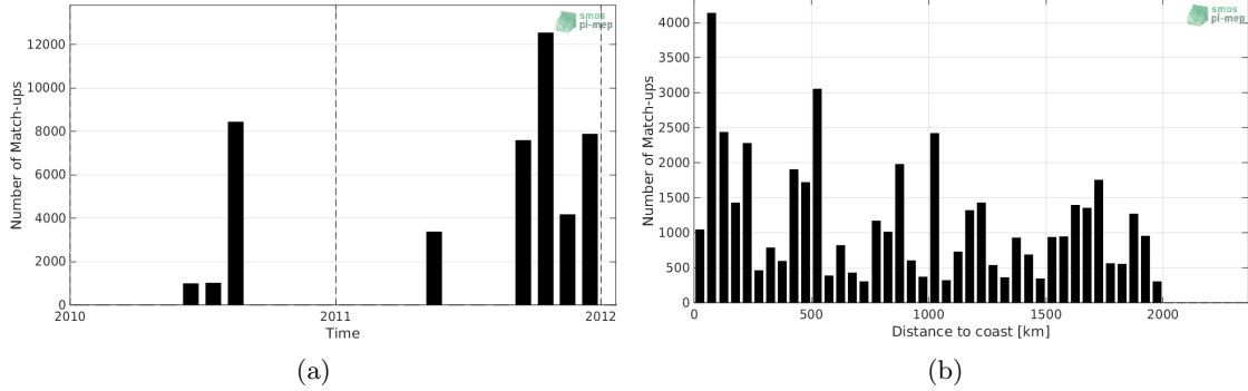
Figure 1: Number of match-ups between TSG-GOSUD-Sailing-ship and SMOS-L2-DPGS-v662 SSS as a function of time (a) and as function of the distance to coast (b) over the North Pacific Ocean Pi-MEP region and for the full satellite product period.
