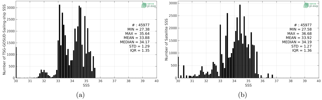
Figure 2: Histograms of SSS from TSG-GOSUD-Sailing-ship (a) and SMOS-L2-DPGS-v662 (b) considering all match-up pairs per bins of 0.1 over the North Pacific Ocean Pi-MEP region and for the full satellite product period.
