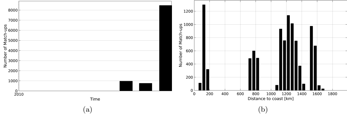
Figure 1: Number of match-ups between TSG-GOSUD-Sailing-ship and SMOS-L2-DPGS-v662 SSS as a function of time (a) and as function of the distance to coast (b) over the North Pacific Ocean Pi-MEP region and for the full satellite product period.
