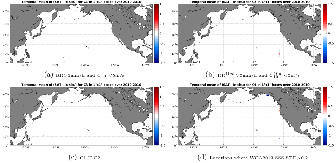
Figure 12: Temporal mean gridded over spatial boxes of size 1^\circ \times 1^\circ of \Delta SSS (SMOS-L2-DPGS-v662 - TSG-GOSUD-Sailing-ship) for 4 different subdatasets corresponding to: RR > 1mm/h and U_{10} < 5 m/s (a), RR^{10d} > 5 mm/h and U_{10}^{10d} < 5 m/s (b), C1 U C2 (c), Locations where WOA2013 SSS STD > 0.2 (d).
