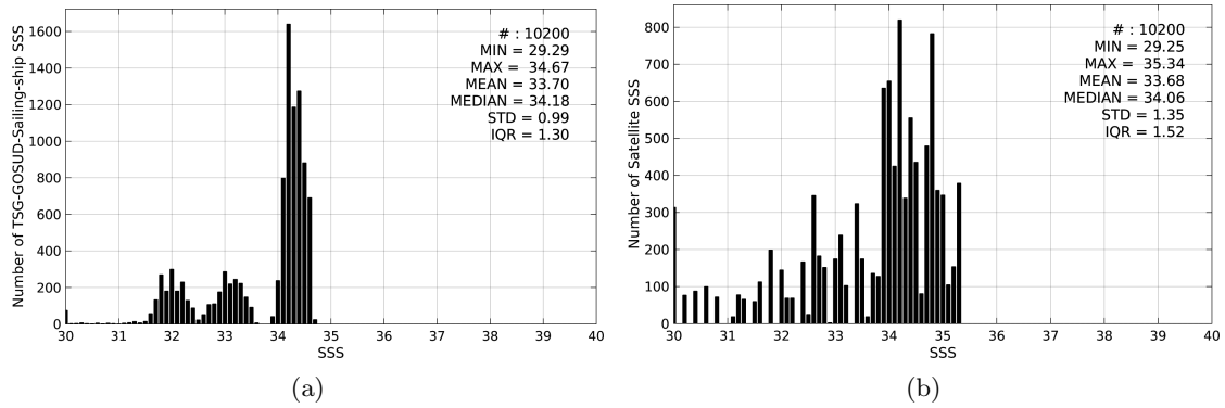
Figure 2: Histograms of SSS from TSG-GOSUD-Sailing-ship (a) and SMOS-L2-DPGS-v662 (b) considering all match-up pairs per bins of 0.1 over the North Pacific Ocean Pi-MEP region and for the full satellite product period.
