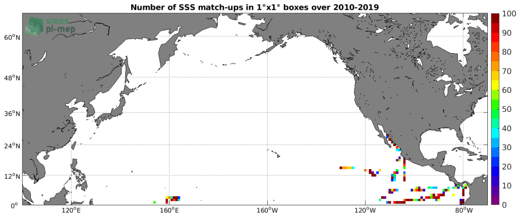
Figure 4: Number of SSS match-ups between TSG (GOSUD-Research-vessel) SSS and the SMOS SSS L2 v662 (ESA) SSS product for the North Pacific Ocean Pi-MEP region over 1°x1° boxes and for the full satellite product period.
