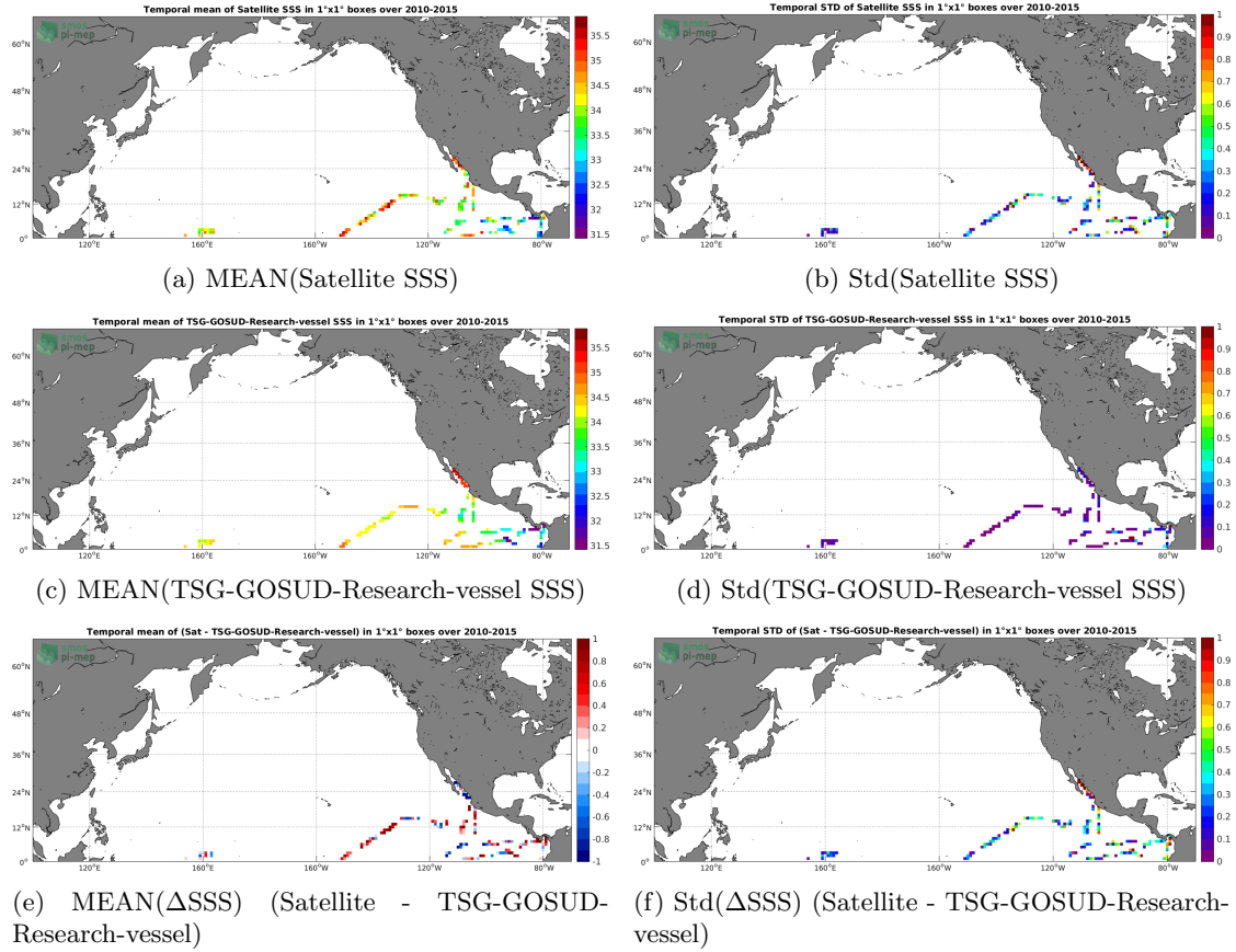
Figure 6: Temporal mean (left) and Std (right) of SSS from SMOS L2 v662 (ESA) (top), TSG-GOSUD-Research-vessel (middle), and of \Delta SSS (Satellite - TSG-GOSUD-Research-vessel). Only match-up pairs are used to generate these maps.
