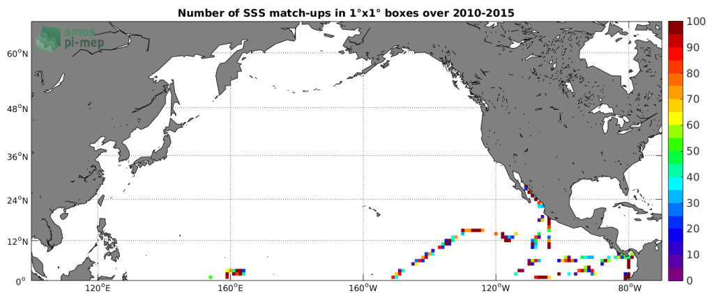
Figure 4: Number of SSS match-ups between TSG-GOSUD-Research-vessel SSS and the SMOS L2 v662 (ESA) SSS product for the North Pacific Ocean Pi-MEP region over 1^\circ \times 1^\circ boxes and for the full satellite product period.
