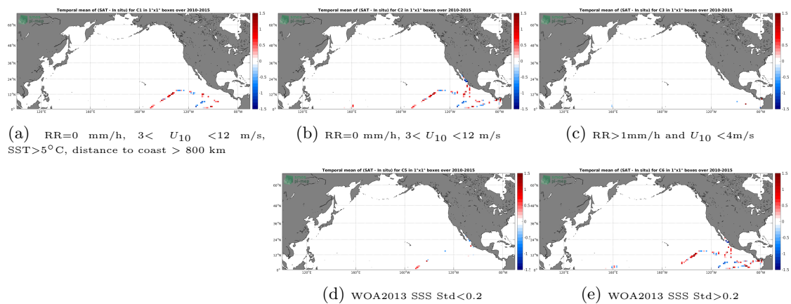
Figure 12: Temporal mean gridded over spatial boxes of size 1^\circ \times 1^\circ of \Delta SSS (SMOS L2 v662 (ESA) - TSG-GOSUD-Research-vessel) for 5 different subdatasets corresponding to:RR=0 mm/h, 3 < U_{10} < 12 m/s, SST >5^\circ\text{C} , distance to coast > 800 km (a), RR=0 mm/h, 3 < U_{10} < 12 m/s (b), RR >1 mm/h and U_{10} < 4 m/s (c), WOA2013 SSS Std <0.2 (d), WOA2013 SSS Std >0.2 (e).
