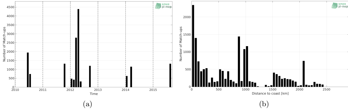
Figure 1: Number of match-ups between TSG-GOSUD-Research-vessel and SMOS L2 v662 (ESA) SSS as a function of time (a) and as function of the distance to coast (b) over the North Pacific Ocean Pi-MEP region and for the full satellite product period.
