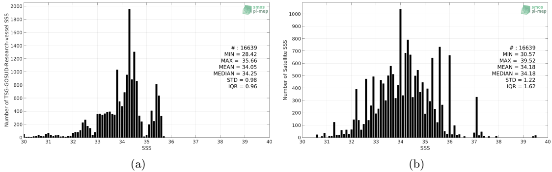
Figure 2: Histograms of SSS from TSG-GOSUD-Research-vessel (a) and SMOS L2 v662 (ESA) (b) considering all match-up pairs per bins of 0.1 over the North Pacific Ocean Pi-MEP region and for the full satellite product period.
