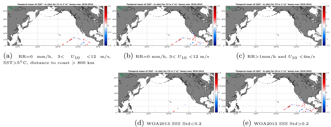
Figure 12: Temporal mean gridded over spatial boxes of size 1^\circ \times 1^\circ of \Delta SSS (SMOS-L2-DPGS-v662 - TSG-GOSUD-Research-vessel) for 5 different subdatasets corresponding to:RR=0 mm/h, 3 < U_{10} < 12 m/s, SST > 5^\circ\text{C} , distance to coast > 800 km (a), RR=0 mm/h, 3 < U_{10} < 12 m/s (b), RR > 1 mm/h and U_{10} < 4 m/s (c), WOA2013 SSS Std < 0.2 (d), WOA2013 SSS Std > 0.2 (e).
