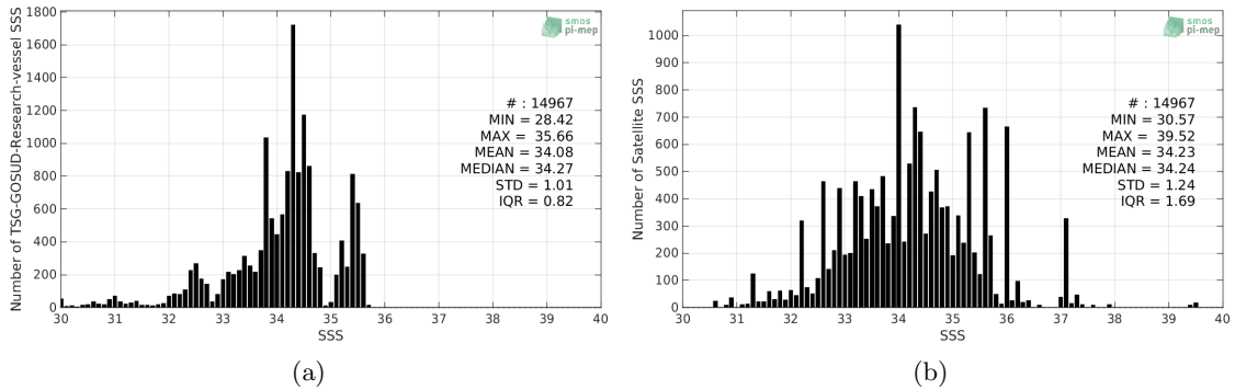
Figure 2: Histograms of SSS from TSG-GOSUD-Research-vessel (a) and SMOS-L2-DPGS-v662 (b) considering all match-up pairs per bins of 0.1 over the North Pacific Ocean Pi-MEP region and for the full satellite product period.
