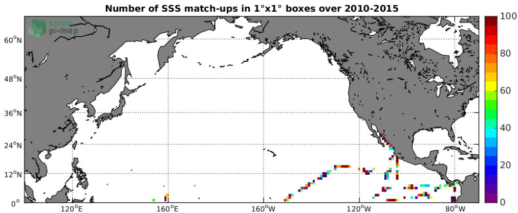
Figure 4: Number of SSS match-ups between TSG-GOSUD-Research-vessel SSS and the SMOS-L2-DPGS-v662 SSS product for the North Pacific Ocean Pi-MEP region over 1°x1° boxes and for the full satellite product period.
