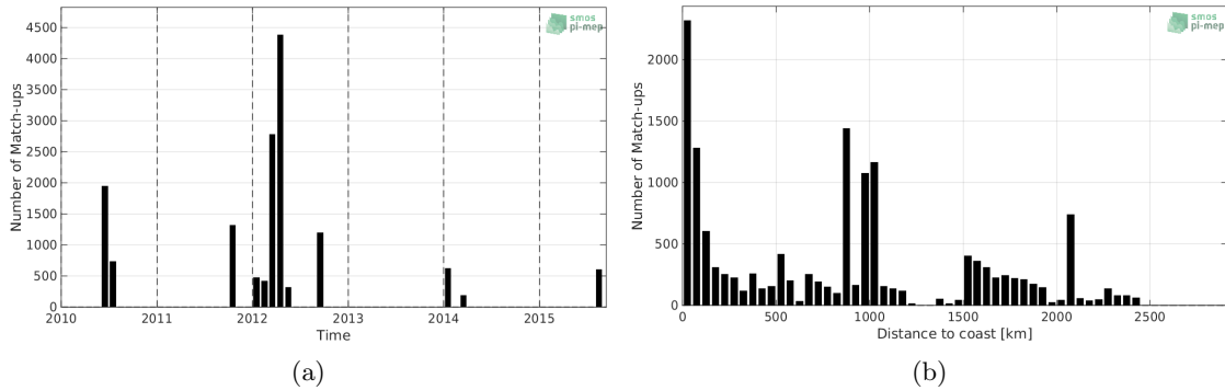
Figure 1: Number of match-ups between TSG-GOSUD-Research-vessel and SMOS-L2-DPGS-v662 SSS as a function of time (a) and as function of the distance to coast (b) over the North Pacific Ocean Pi-MEP region and for the full satellite product period.
