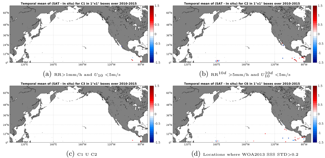
Figure 12: Temporal mean gridded over spatial boxes of size 1^\circ \times 1^\circ of \Delta SSS (SMOS-L2-DPGS-v662 - TSG-GOSUD-Research-vessel) for 4 different subdatasets corresponding to: RR > 1\text{mm/h} and U_{10} < 5\text{m/s} (a), RR^{10d} > 5\text{mm/h} and U_{10}^{10d} < 5\text{m/s} (b), C1 \cup C2 (c), Locations where WOA2013 SSS STD > 0.2 (d).
