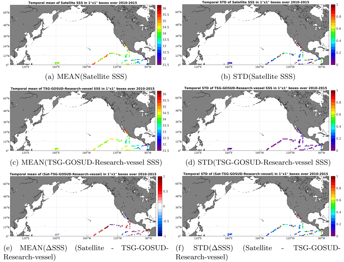
Figure 6: Temporal mean (left) and STD (right) of SSS from SMOS-L2-DPGS-v662 (top), TSG-GOSUD-Research-vessel (middle), and of \Delta SSS (Satellite - TSG-GOSUD-Research-vessel). Only match-up pairs are used to generate these maps.
