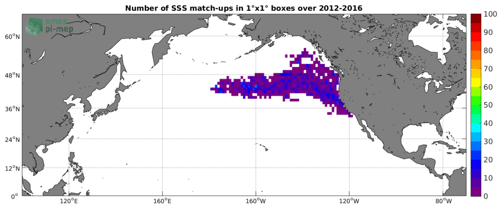
Figure 4: Number of SSS match-ups between Sea mammals SSS and the SMOS SSS L2 v662 (ESA) SSS product for the North Pacific Ocean Pi-MEP region over 1^\circ \times 1^\circ boxes and for the full satellite product period.
