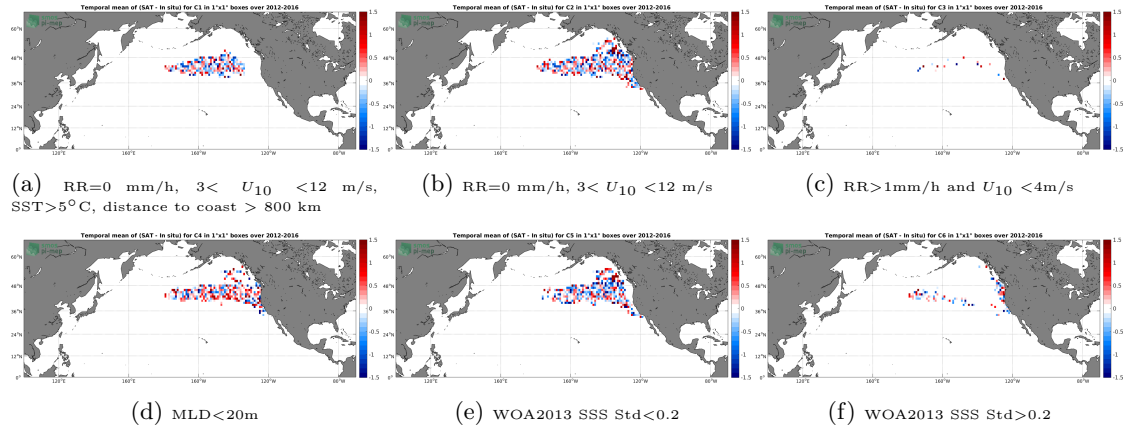
Figure 12: Temporal mean gridded over spatial boxes of size 1^\circ \times 1^\circ of \Delta SSS (SMOS SSS L2 v662 (ESA) - Sea mammals) for 6 different subdatasets corresponding to: RR=0 mm/h, 3 < U_{10} < 12 m/s, SST > 5^\circ C , distance to coast > 800 km (a), RR=0 mm/h, 3 < U_{10} < 12 m/s (b), RR > 1 mm/h and U_{10} < 4 m/s (c), MLD < 20 m (d), WOA2013 SSS Std < 0.2 (e), WOA2013 SSS Std > 0.2 (f).
