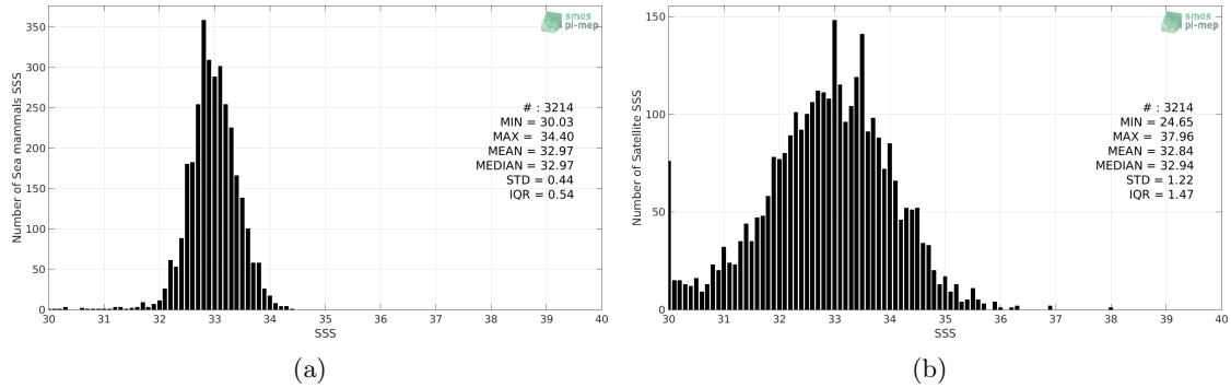
Figure 2: Histograms of SSS from Sea mammals (a) and SMOS SSS L2 v662 (ESA) (b) considering all match-up pairs per bins of 0.1 over the North Pacific Ocean Pi-MEP region and for the full satellite product period.
