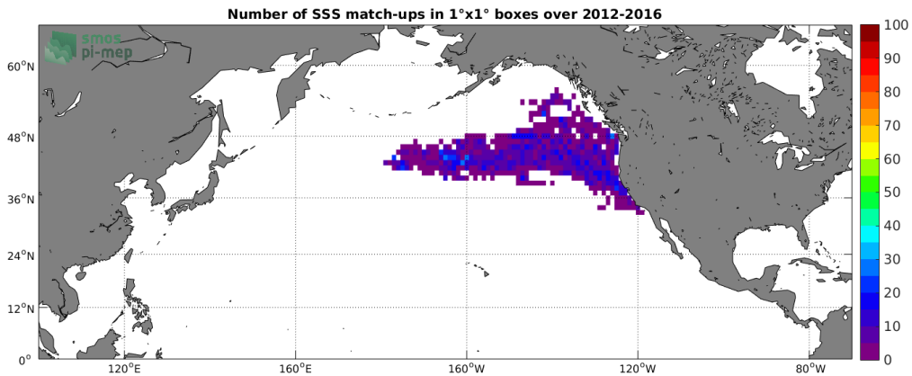
Figure 4: Number of SSS match-ups between Sea mammals SSS and the SMOS SSS L2 v662 (ESA) SSS product for the North Pacific Ocean Pi-MEP region over 1°x1° boxes and for the full satellite product period.
