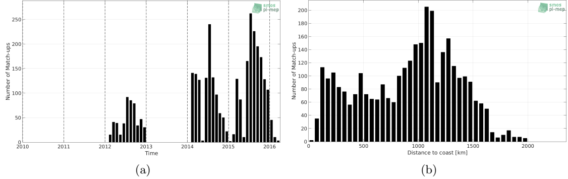
Figure 1: Number of match-ups between Sea mammals and SMOS SSS L2 v662 (ESA) SSS as a function of time (a) and as function of the distance to coast (b) over the North Pacific Ocean Pi-MEP region and for the full satellite product period.
