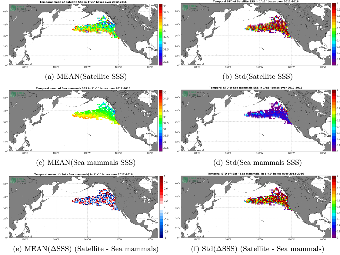
Figure 6: Temporal mean (left) and Std (right) of SSS from SMOS SSS L2 v662 (ESA) (top), Sea mammals (middle), and of \Delta SSS (Satellite - Sea mammals). Only match-up pairs are used to generate these maps.
