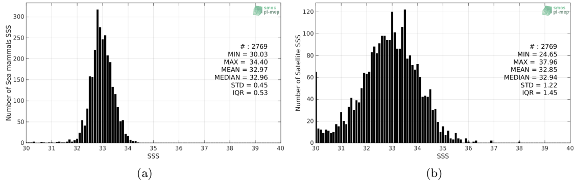
Figure 2: Histograms of SSS from Sea mammals (a) and SMOS-L2-DPGS-v662 (b) considering all match-up pairs per bins of 0.1 over the North Pacific Ocean Pi-MEP region and for the full satellite product period.
