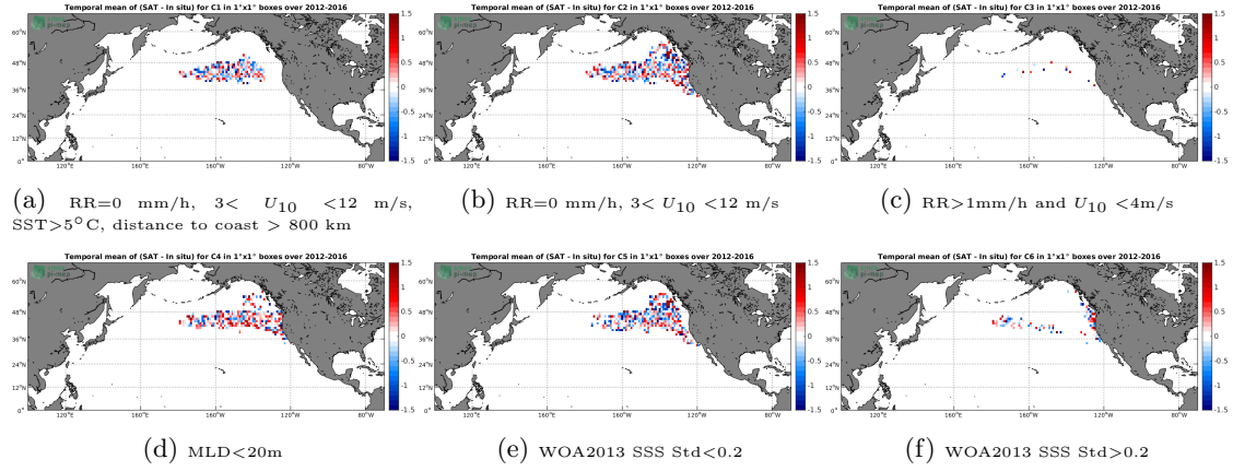
Figure 12: Temporal mean gridded over spatial boxes of size 1^\circ \times 1^\circ of \Delta SSS (SMOS-L2-DPGS-v662 - Sea mammals) for 6 different subdatasets corresponding to: RR=0 mm/h, 3 < U_{10} < 12 m/s, SST >5^\circ\text{C} , distance to coast > 800 km (a), RR=0 mm/h, 3 < U_{10} < 12 m/s (b), RR >1 mm/h and U_{10} < 4 m/s (c), MLD <20 m (d), WOA2013 SSS Std <0.2 (e), WOA2013 SSS Std >0.2 (f).
