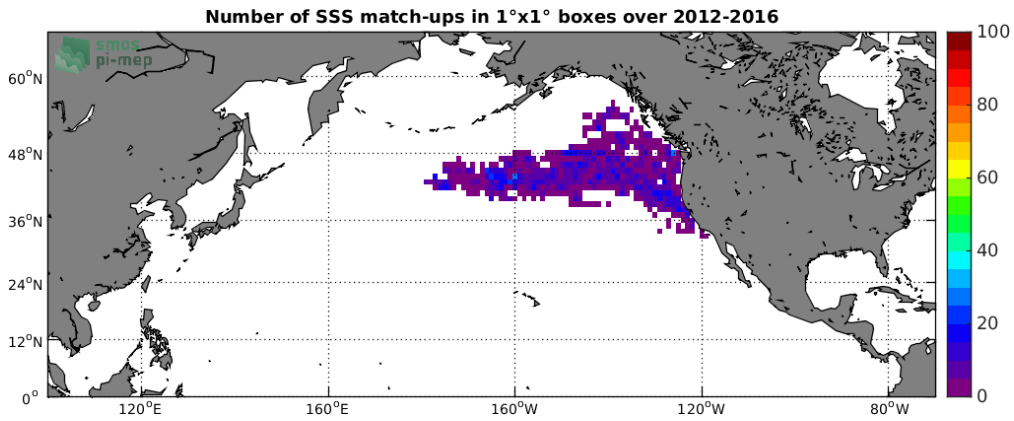
Figure 4: Number of SSS match-ups between Sea mammals SSS and the SMOS-L2-DPGS-v662 SSS product for the North Pacific Ocean Pi-MEP region over 1°x1° boxes and for the full satellite product period.
