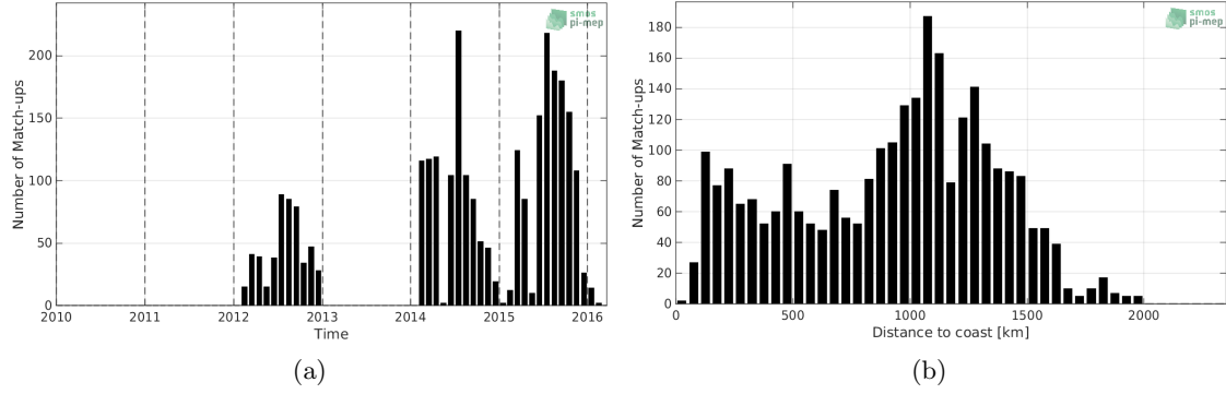
Figure 1: Number of match-ups between Sea mammals and SMOS-L2-DPGS-v662 SSS as a function of time (a) and as function of the distance to coast (b) over the North Pacific Ocean Pi-MEP region and for the full satellite product period.
