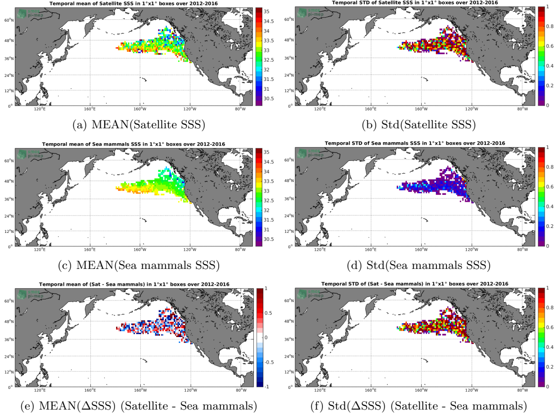
Figure 6: Temporal mean (left) and Std (right) of SSS from SMOS-L2-DPGS-v662 (top), Sea mammals (middle), and of \Delta SSS (Satellite - Sea mammals). Only match-up pairs are used to generate these maps.
