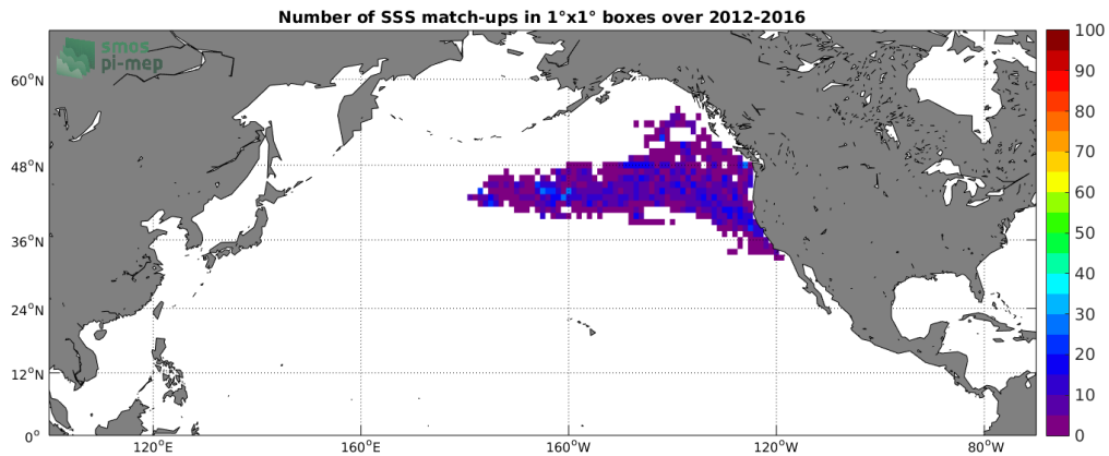
Figure 4: Number of SSS match-ups between Sea mammals SSS and the SMOS-L2-DPGS-v662 SSS product for the North Pacific Ocean Pi-MEP region over 1^\circ \times 1^\circ boxes and for the full satellite product period.
